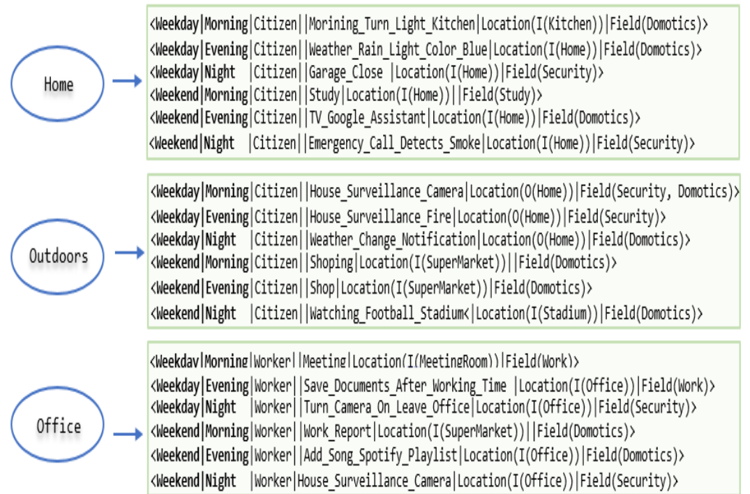
Figure 12. An example of a user rules repository in three user’s domains.
