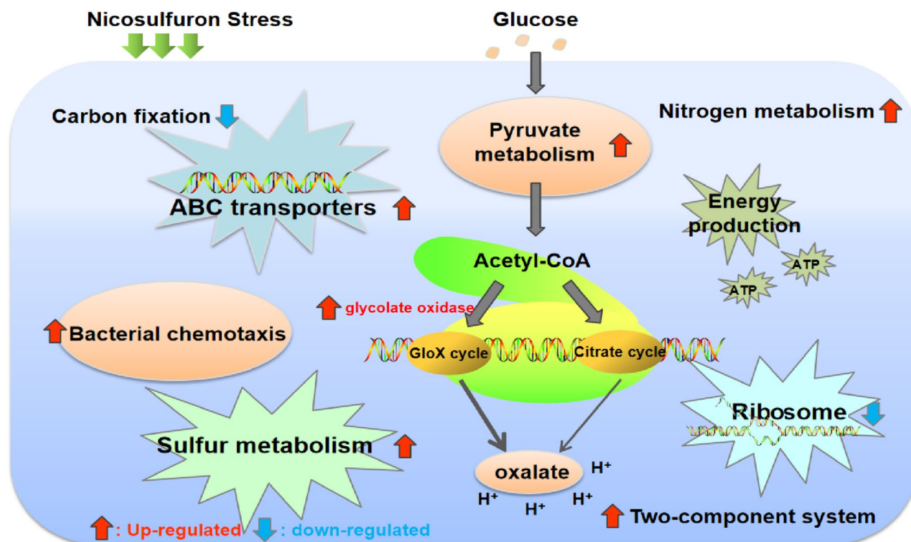
Figure 5. Transcriptional responses of Pseudomonas nicosulfuronedens LAM1902 to nicosulfuron. ↑: the number of up-regulated genes > the number of down-regulated genes, ↓: the number of up-regulated genes < the number of down-regulated genes.
