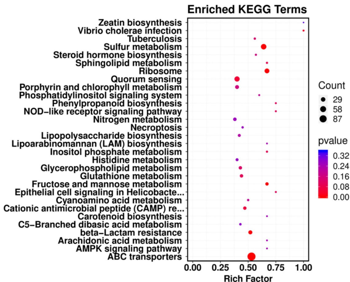
Figure 4. The differentially expressed genes enriched in KEGG pathways during nicosulfuron degradation by Pseudomonas nicosulfuronedens LAM1902 45 .
