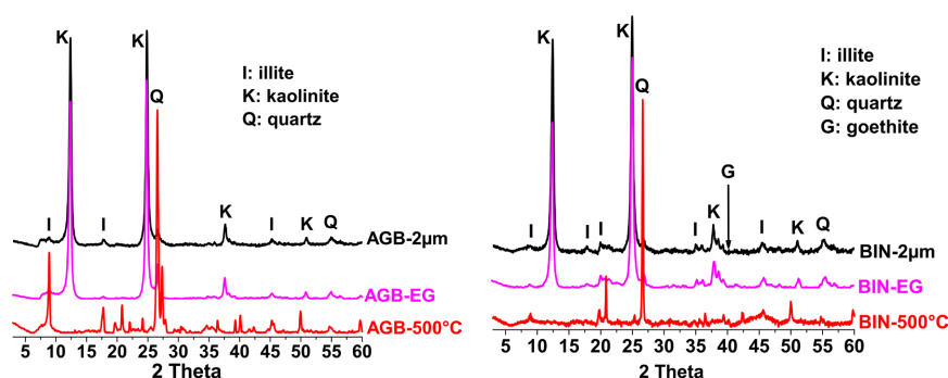
Figure 4. X-ray diffractograms of oriented preparations of AGB and BIN clays (2 \mu\text{m} : fine clay fraction at 2 \mu\text{m} ; EG: ethylene glycol and clays heated to 500°C).
