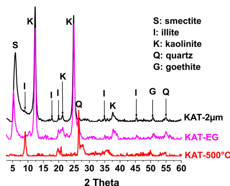
Figure 5. X-ray diffractograms of oriented KAT clay preparations (2 \mu\text{m} : fine clay fraction at 2 \mu\text{m} ; EG: ethylene glycol and KAT heated to 500°C).
