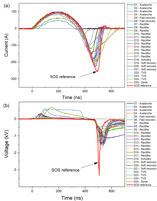
Fig. 3. Current (a) and voltage (b) waveforms of the tested off-the-shelf diodes in comparison with the SOS reference diode.
