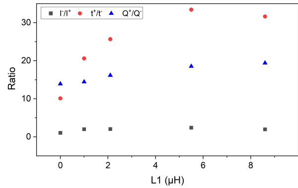
Fig. 10. Ratios of the pumping currents (square), pumping times (round) and electric charges (triangle) as a function of the inductance L1 obtained for the OTS-100 at the resistive load R = 50 \Omega and charging voltage V_{C1} = 6 kV.
