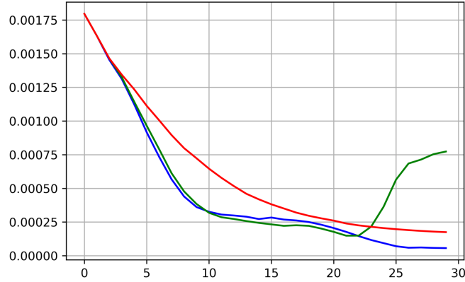
Figure 1: Decrease of the functional J . Blue: adaptive restart, green: Nesterov's, red: gradient descent.
