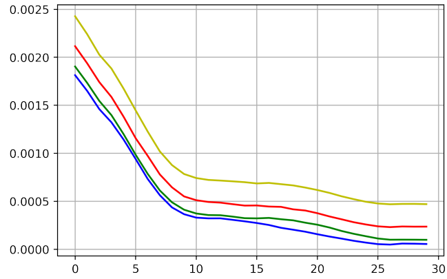
Figure 6: Decrease of the functional F_0 for noise levels. Blue: 1%, green: 2.5%, red: 5%, yellow: 7.5%.
