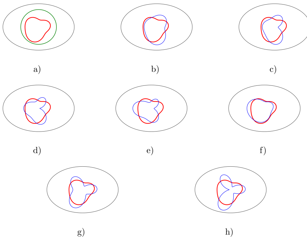
Figure 2: Nesterov's method. Exact - red, initial - green and approximate - blue solutions for different iterations: a) initial position, b) 4 iteration, c) 8 iteration, d) 12 iteration, e) 16 iteration, f) 20 iteration, g) 24 iteration, h) 30 iteration.
