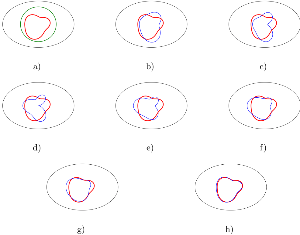
Figure 3: Adaptive restart method. Red: exact, green: initial and blue: approximate solutions for different iterations: a) initial position, b) 4 iteration, c) 8 iteration, d) 12 iteration, e) 16 iteration, f) 20 iteration, g) 24 iteration, h) 30 iteration.
