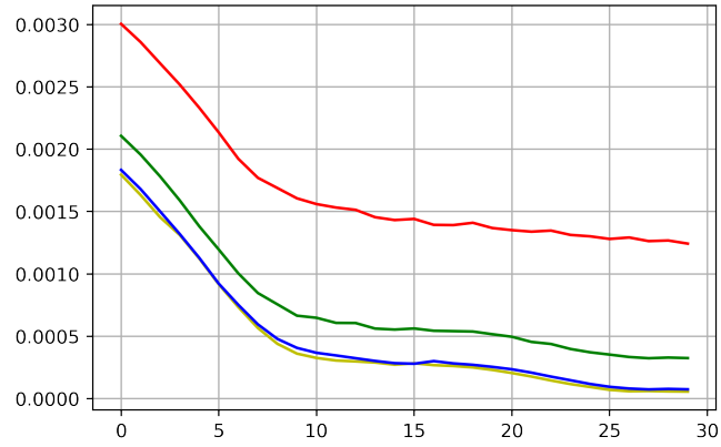
Figure 4: Decrease of the functional J for noise levels. Yellow: 0%, blue: 1%, green: 2.5%, red: 5%.
