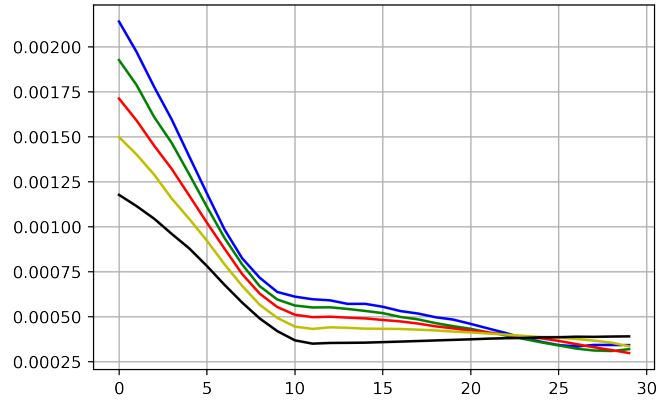
Figure 8: Decrease of the functional F_\alpha for noise level 5% with different \alpha . Blue: 0, green: 0.1, red: 0.2, yellow: 0.3, black: 0.4.
