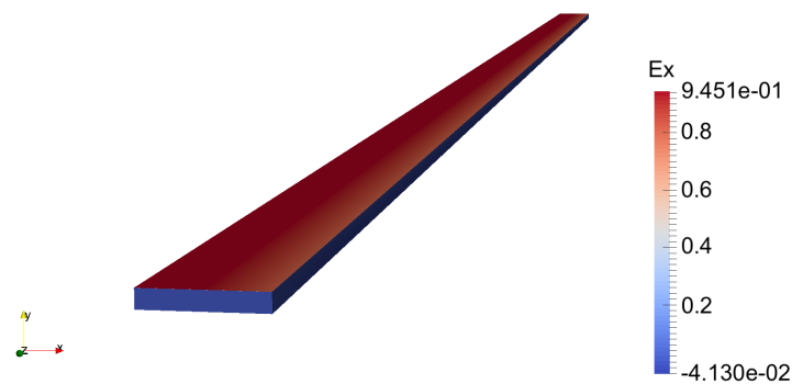
Figure 3. Simulated electric field when the incident field is polarized in the normal direction with respect to the fibers for \omega_2 = 24.5 GHz.
