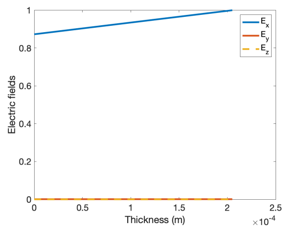
Figure 4. Through-the-thickness-simulated electric field when the incident field is polarized in the normal direction with respect to the fibers for \omega_1 = 2.45 GHz.
