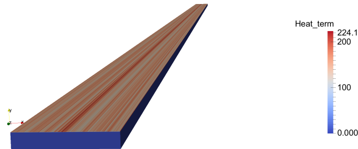
Figure 13. Heat-generation source (in \text{W}/\text{m}^3 ) for \omega_1 = 2.45 GHz and the incident electric field polarized in the normal direction with respect to the fiber orientation.
