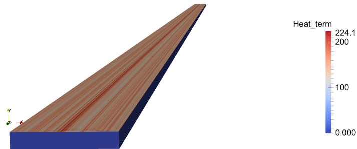
Figure 13. Heat-generation source (in W/m^3 ) for \omega_1 = 2.45 GHz and the incident electric field polarized in the normal direction with respect to the fiber orientation.
