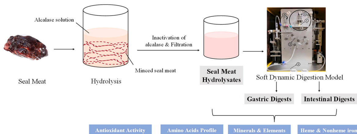
Fig. 1. Scheme of the generation, digestion, and analyses of seal meat hydrolysates.
