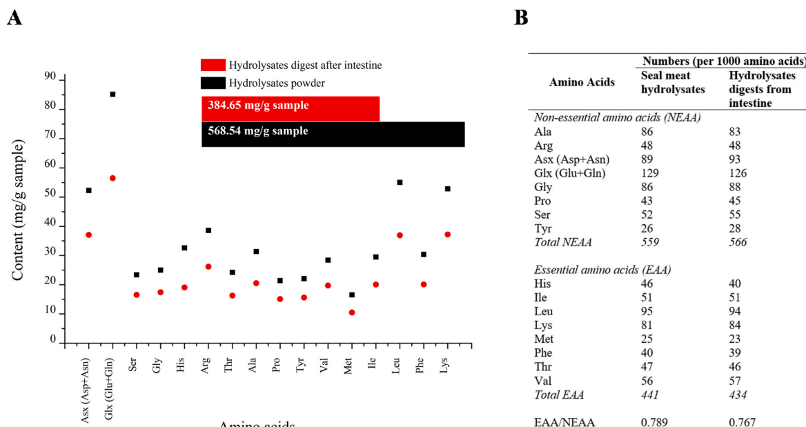
Fig. 2. Protein and amino acids profiles. (A) Content of amino acids (mg/g sample) of seal meat hydrolysates and its intestinal digests. (B) Amino acids composition (number per 1000 amino acids) of seal meat hydrolysates and its intestinal digests.
