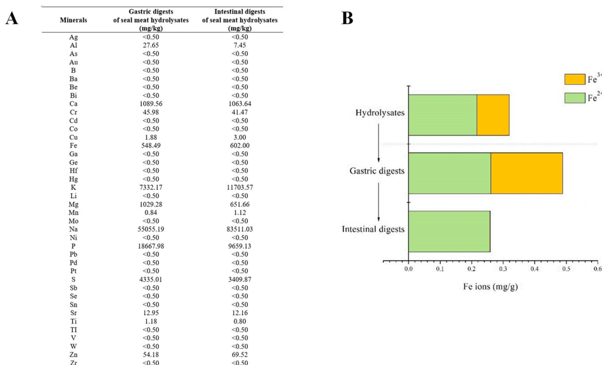
Fig. 3. (A) Amounts of minerals (mg/kg) in gastric and intestinal digests of seal meat hydrolysates. (B) Amounts of Fe 2+ and Fe 3+ ions (mg/g) in seal meat hydrolysates and its gastric and intestinal digests.
