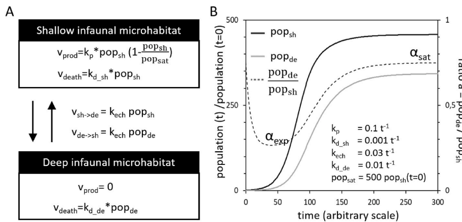
Fig. 2. A. Deterministic model to explain these relations based on bioturbation and chemotaxis forcing. v_{\text{prod}} , v_{\text{death}} , v_{\text{sh} \rightarrow \text{de}} and v_{\text{de} \rightarrow \text{sh}} correspond to the rate of reproduction, the rate of death, the rate of exchange from shallow to deep microhabitat and the rate of exchange from deep to shallow microhabitat respectively. k_p , k_{d_{\text{sh}}} , k_{d_{\text{de}}} and k_{\text{ech}} are the associated parameters while \text{pop}_{\text{sh}} and \text{pop}_{\text{de}} are the population of shallow and deep microhabitat. B. Example of a representative result from the model following a 500 fold increase of environment capability, i. e. 500 fold \text{pop}_{\text{sat}} increase.
