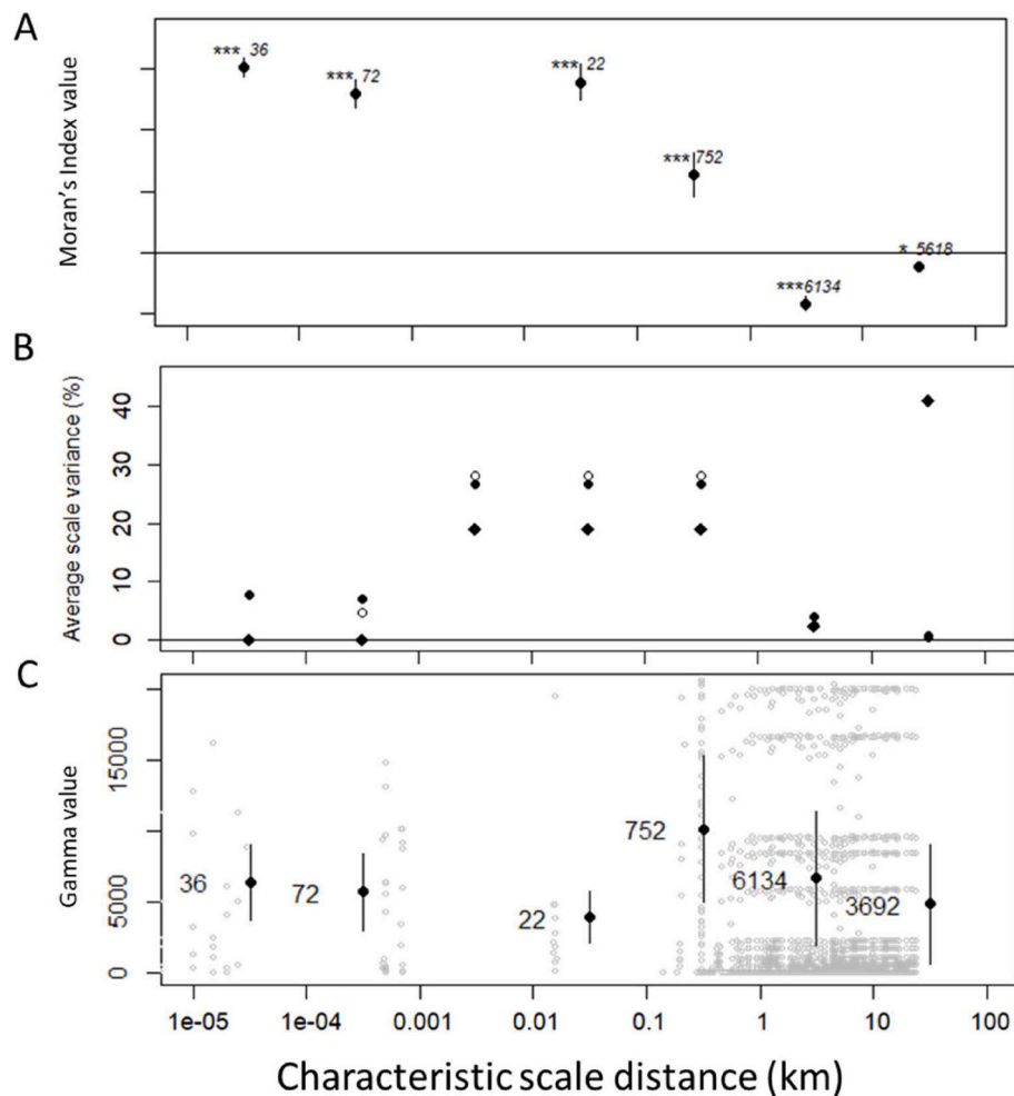
Fig. 4. Geostatistical model processes with the dataset from Fig. 1 (black dots).
