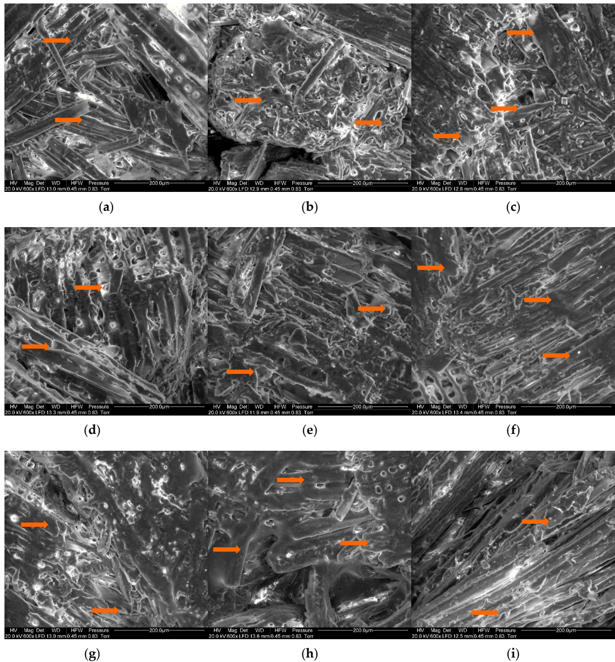
Figure 6. Scanning electron microscope images of lignocellulosic composites with (a) PLA12, (b) PLA15, (c) PLA20, (d) PCL12, (e) PCL15, (f) PCL20, (g) PS12, (h) PS20, (i) UF12; zones covered by binder indicated by arrows.
