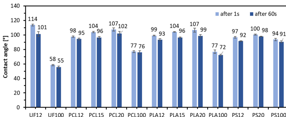
Figure 8. The contact angle of tested lignocellulosic composites and pure binders.
