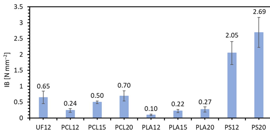
Figure 4. Internal bond (IB) of tested lignocellulosic composites.
