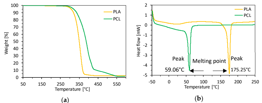
Figure 1. PLA and PCL (a) thermogravimetric analysis (TGA), and (b) differential scanning calorimetry (DSC).
