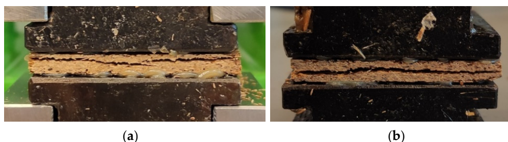
Figure 5. Two representative forms of damage after the IB test (a) near-surface zone (b) in the core layer.
