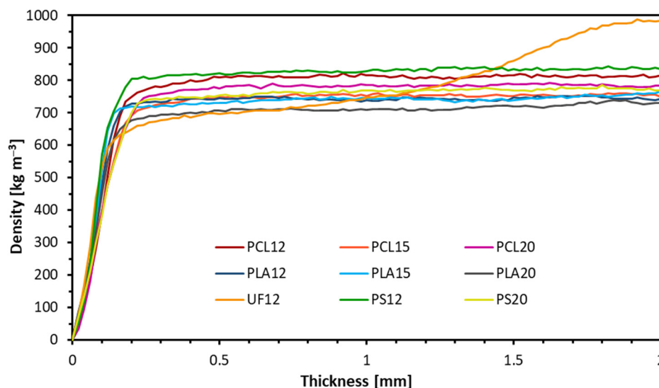
Figure 2. Density profiles of manufactured lignocellulosic composites.
