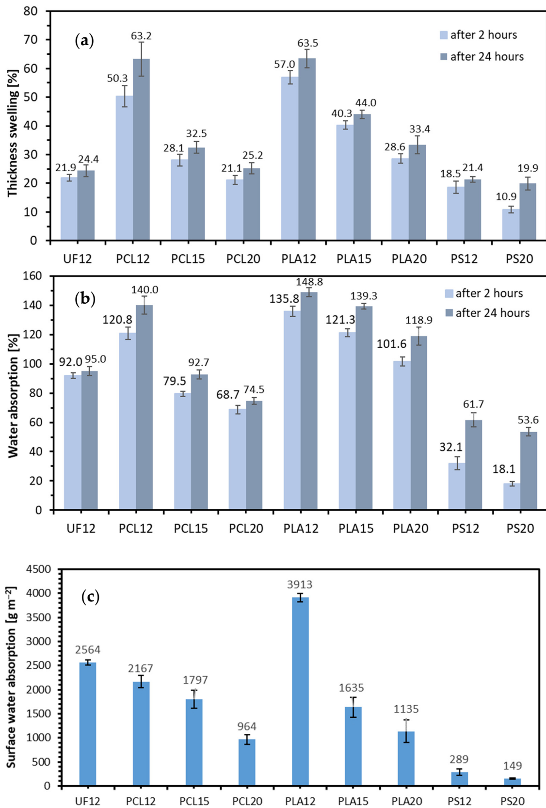
Figure 7. (a) Thickness swelling, (b) water absorption, and (c) surface water absorption of tested lignocellulosic composites.
