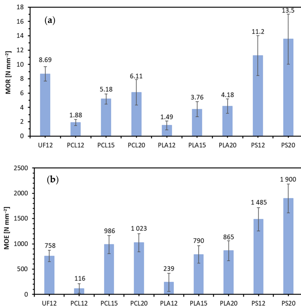
Figure 3. (a) Modulus of rupture (MOR) and (b) modulus of elasticity (MOE) of tested lignocellulosic composites.
