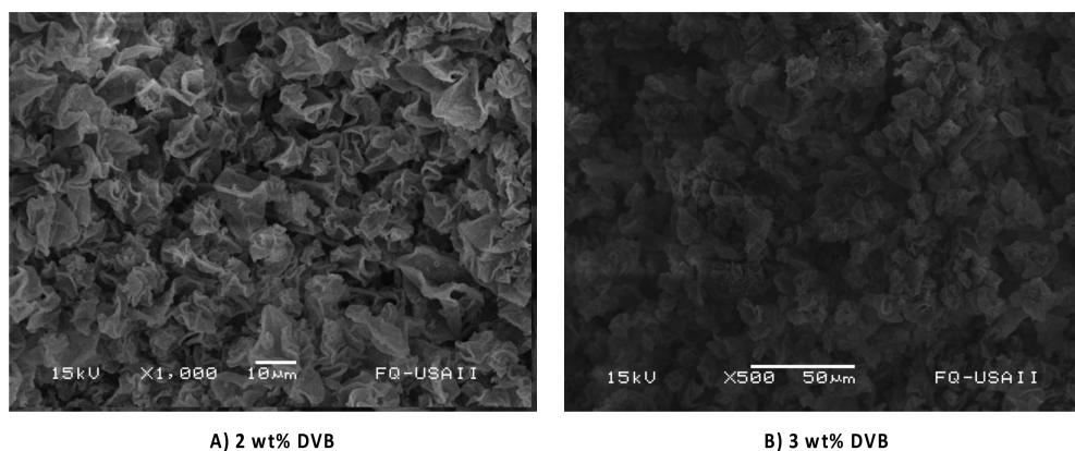
Figure 5. SEM images of hybrid monoliths with bi-continuous morphology, (A) 2 wt% DVB; (B) 3 wt% DVB.
