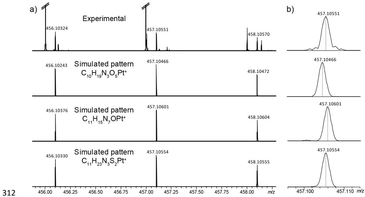
313 Figure 3: MALDI FTICR MS spectra of (a) Experimental and theoretical isotopic 314 distribution patterns of C 10 H 19 N 3 O 5 Pt, C 11 H 15 N 7 OPt and C 11 H 23 N 3 S 2 Pt for M ( 194 Pt), M+1 315 ( 195 Pt) and M+2 ( 196 Pt) isotopes (b) expanded m/z window of the experimental monoisotopic 316 peak at m/z 457,10551 and the three theoretical monoisotopic peaks of C 10 H 19 N 3 O 5 Pt, 317 C 11 H 15 N 7 OPt and C 11 H 23 N 3 S 2 Pt. 318
