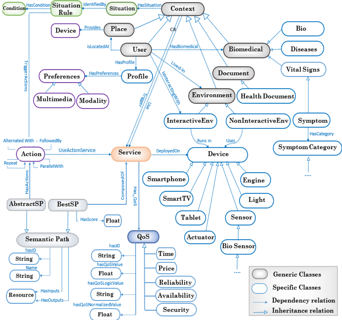
Figure 1. CxQSHHealthOnto Ontology Model
