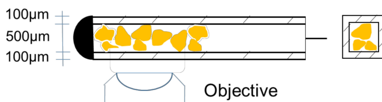
Figure 1. Experimental setup for optical microscopy runs. The cell, a thin glass capillary with a square cross-section, is inserted into a thermostated holder (not shown), on an inverted microscope.
