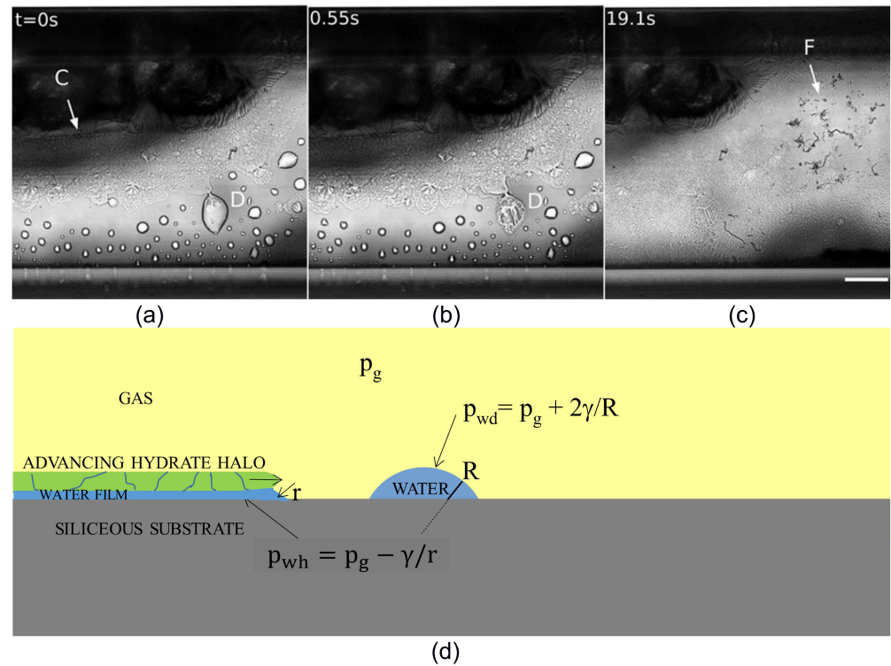
Figure 6. A halo and filaments of methane hydrate observed during a second cycle, at 4\ ^\circ\text{C} , 7\ \text{MPa} in run 5 on the optical microscope. Images a, b and c are extracted from the Supplementary Materials Video S1. (a) Growth of the halo on the glass, from the contact line “C”; (b) the halo leapfrogs over a droplet of water on the glass, “D”; (c) a few seconds later, the presence of filaments, “F”; (d) Schematic of the capillary effect causing rapid displacement of water. Scale bar: 100\ \mu\text{m} . p_{wh} is the pressure of the water under the halo; p_{wd} is the pressure of the water in the drop; p_g is the gas pressure; \gamma is the water–methane interfacial tension; R is the radius of the drop; r is the radius of the water film.
