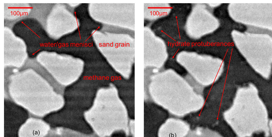
Figure 3. Early stages of methane hydrate growth, results of run 1: (a) Image on reaching 1–2 °C; (b) Methane hydrate is visible in an image taken 0.58 h later.
