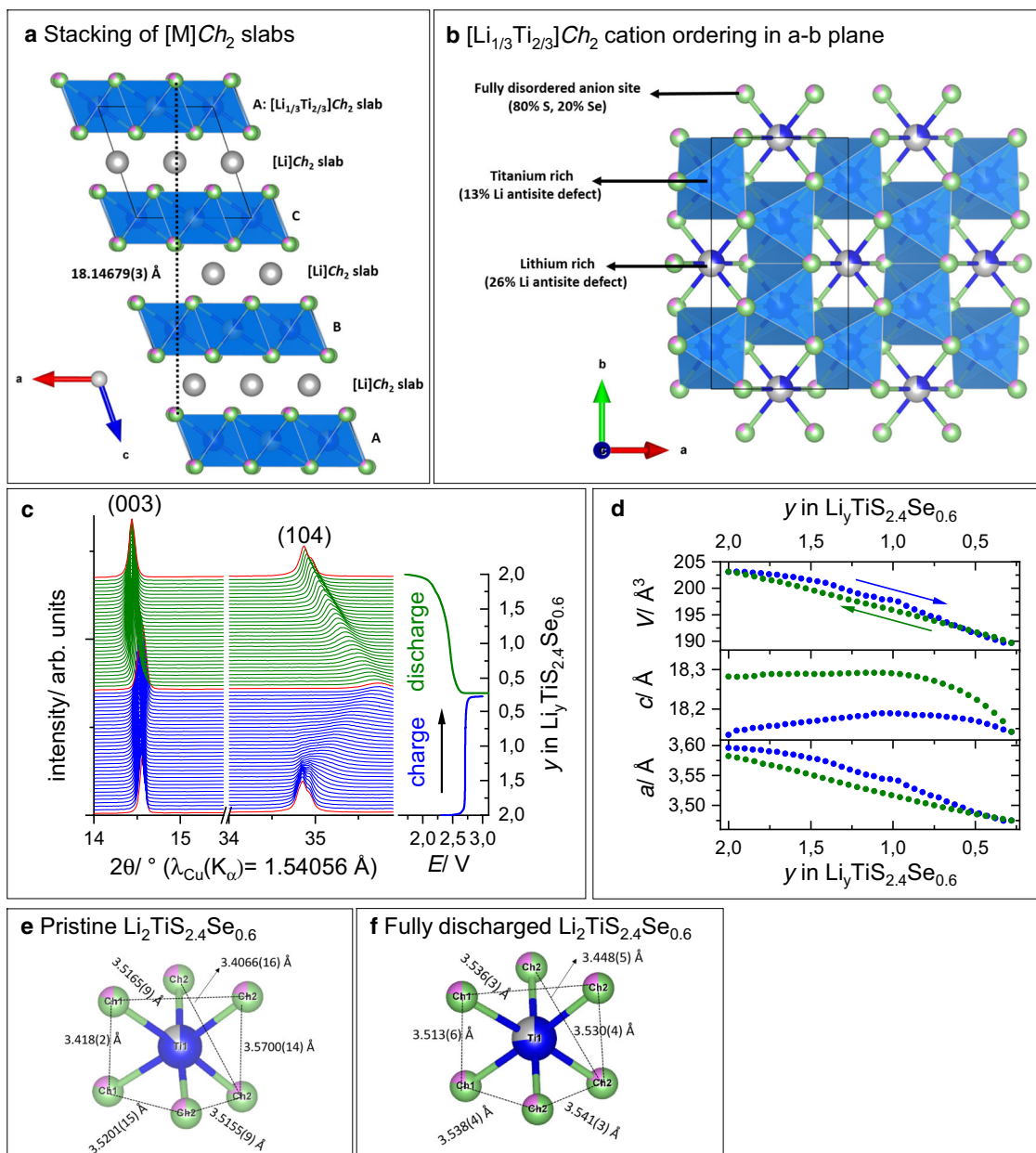
Fig. 3 Crystal structure of \text{Li}_y\text{TiS}_{2.4}\text{Se}_{0.6} . a Structure of \text{Li}_2\text{TiS}_{2.4}\text{Se}_{0.6} shown along the stacking axis: Li and Ti occupy all octahedral interstices present in the cubic close packing of \text{Ch}^{2-} anions. Partial ordering of the cations leads to the formation of [\text{Li}]\text{Ch}_2 and [\text{Li}_{1/3}\text{Ti}_{2/3}]\text{Ch}_2 layers. b Representation of the mixed [\text{Li}_{1/3}\text{Ti}_{2/3}]\text{Ch}_2 slab: the partial ordering of Li vs Ti. c Evolution of the PXRD patterns of \text{Li}_y\text{TiS}_{2.4}\text{Se}_{0.6} during the 1st cycle of an operando PXRD experiment. d Corresponding evolution of the lattice parameters of \text{Li}_y\text{TiS}_{2.4}\text{Se}_{0.6} (space group: R\bar{3}m ). e, f Local bonding environments around Ti1 of pristine \text{Li}_2\text{TiS}_{2.4}\text{Se}_{0.6} and fully discharged \text{Li}_2\text{TiS}_{2.4}\text{Se}_{0.6} (color code: blue: Ti, gray: Li, green: S, pink: Se).
