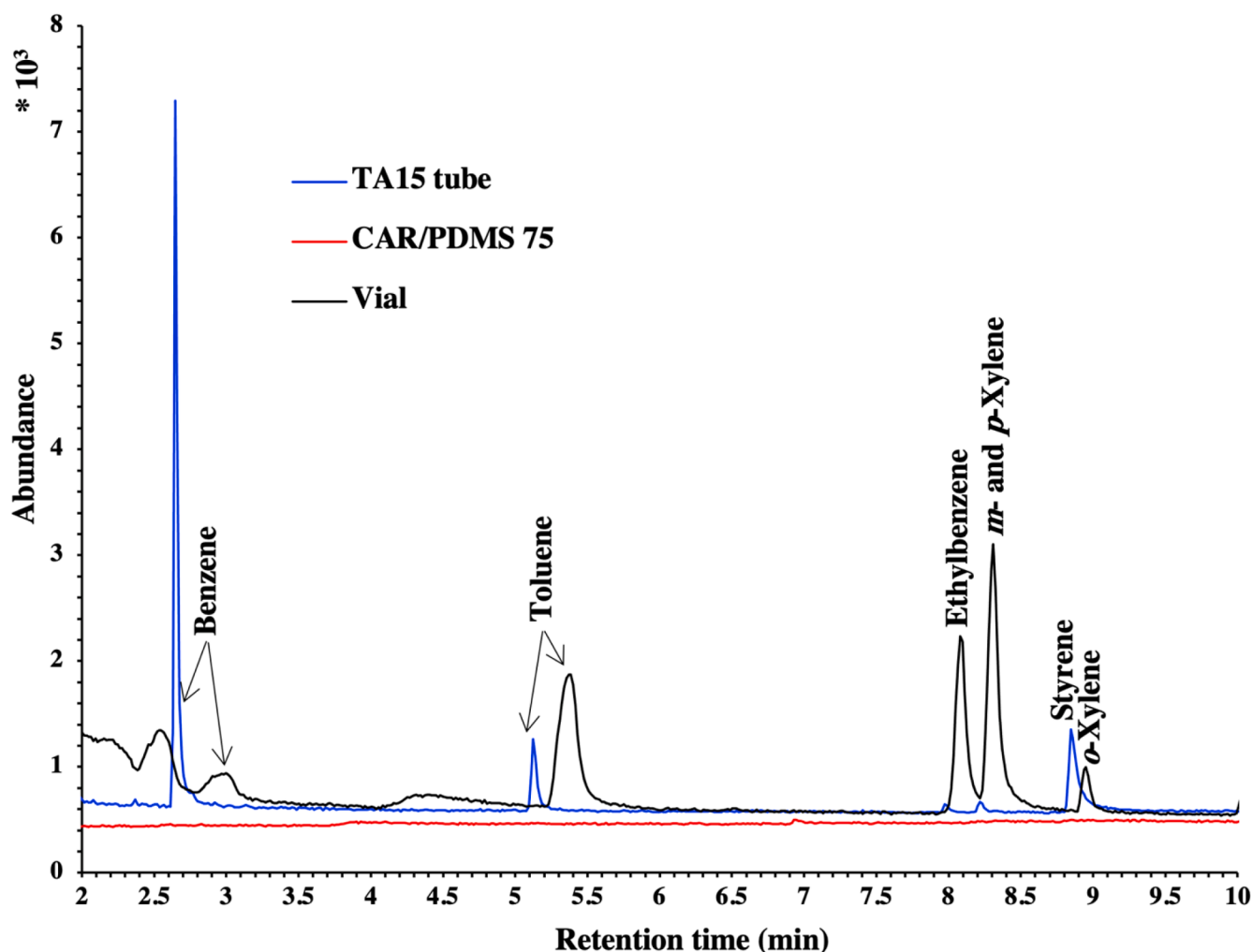
Fig. 6. Total ion current chromatograms of a blank TA15 tube, a blank of the CAR/PDMS 75 \mu\text{m} SPME fiber and a pure CH 4 -filled vial.
