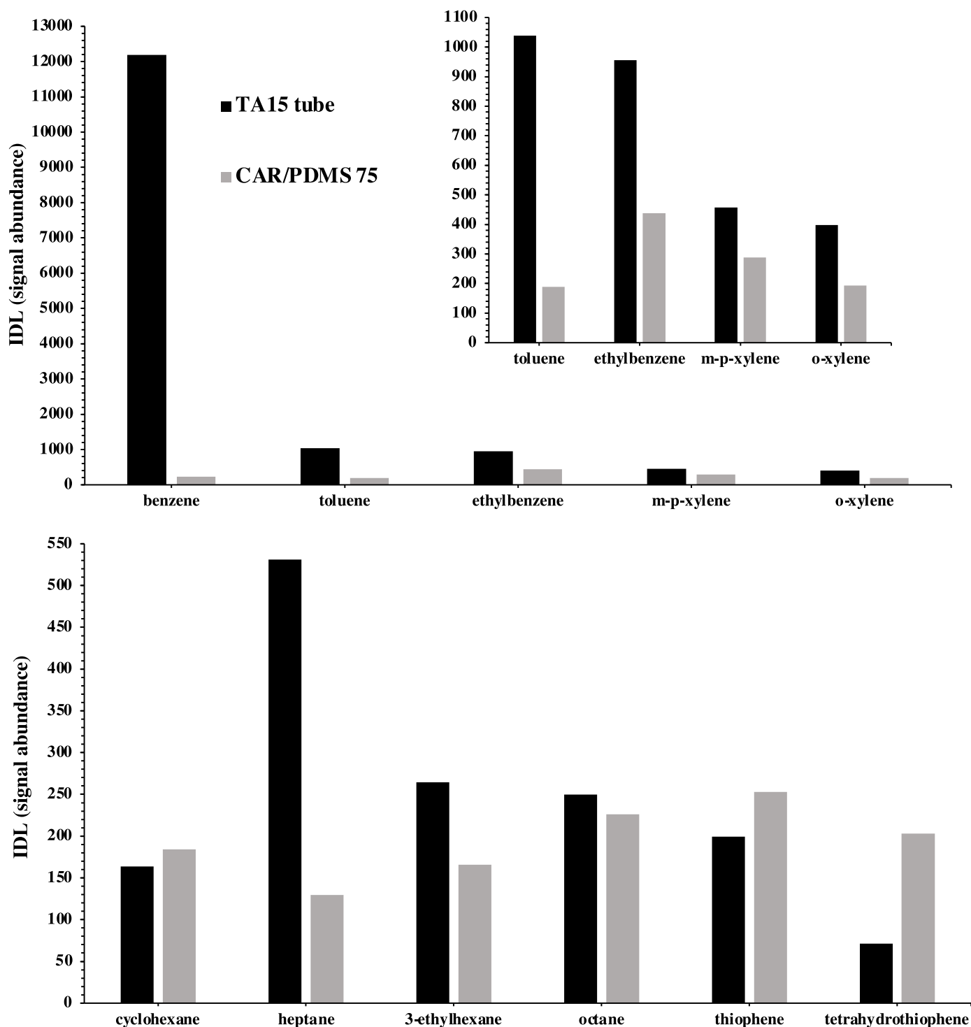
Fig. 7. Instrument detection limits (peak height signal abundance) of trace compounds determined in the NG-A building grid natural gas sample on TA15 tubes and on the CAR/PDMS 75 μm SPME fiber. Numerical values are available in Table S3.
