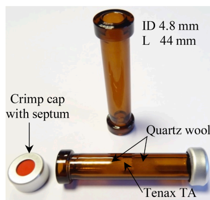
Fig. 2. Custom-built glass tube intended for packing with adsorbents and thermal desorption in the nCx-TD. ID = internal diameter, L = length.
