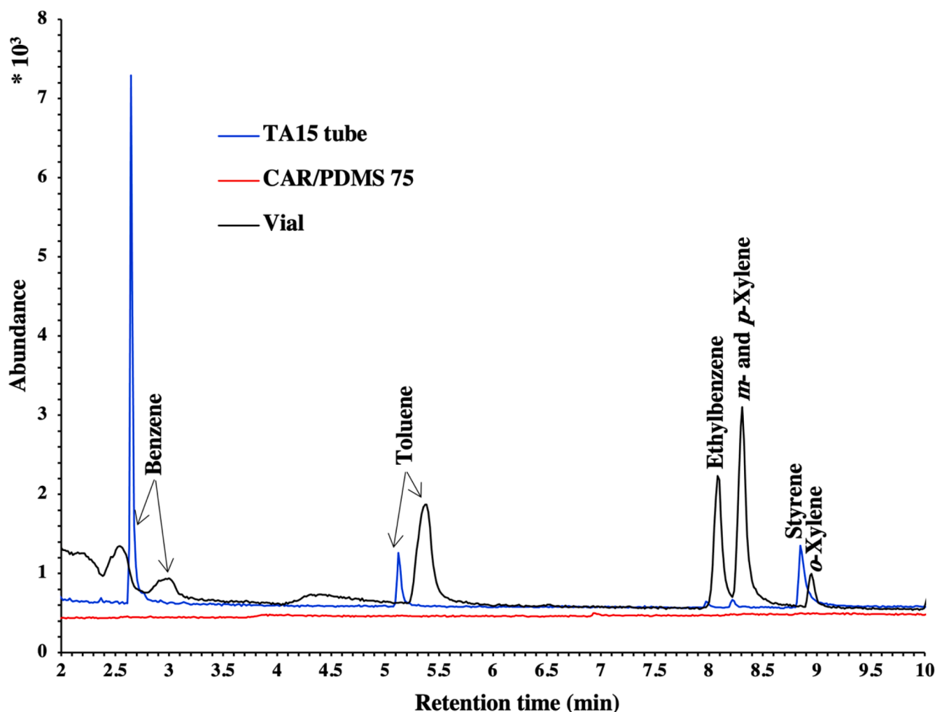
Fig. 6. Total ion current chromatograms of a blank TA15 tube, a blank of the CAR/PDMS 75 \mu\text{m} SPME fiber and a pure \text{CH}_4 -filled vial.
