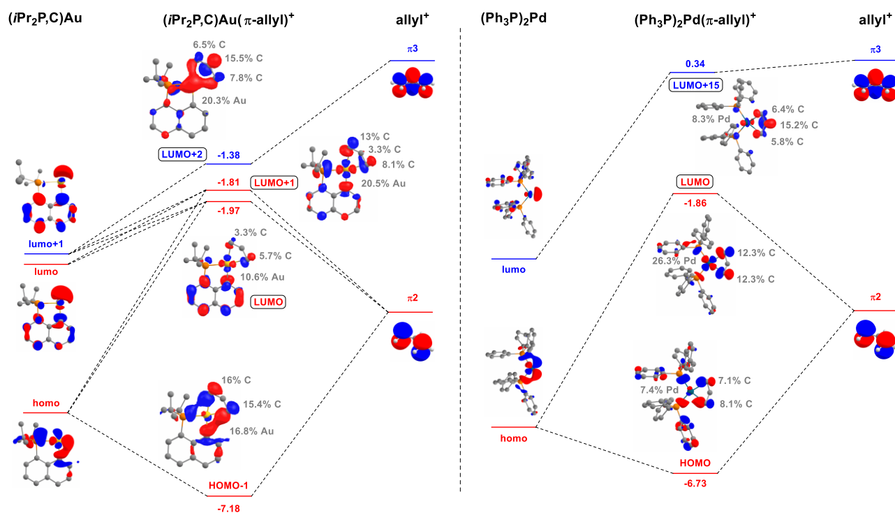
Figure 7. MO diagrams for the Au(III) complex [(\text{P,C})\text{Au}(\pi\text{-allyl})]^+ 2 (left) and its Pd(II) analog [(\text{Ph}_3\text{P})_2\text{Pd}(\pi\text{-allyl})]^+ complex 2-Pd (right) showing the vacant orbitals relevant to nucleophilic additions. Energy of the MOs in eV, cutoff: 0.05. Contribution of the main atoms in each MO in %. Red lines correspond to MOs with large contributions on the terminal carbon atoms of the \pi -allyl moiety while blue lines correspond to MOs with large contributions on the central carbon atom of the \pi -allyl.
