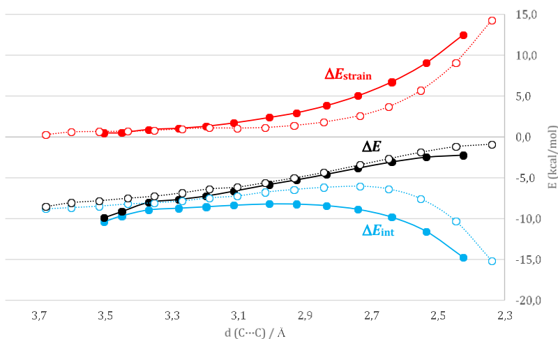
Figure 12. Comparison of the Activation Strain diagrams accounting for the nucleophilic attack of 3b at C_{\text{cent}} (dotted lines) and C_{\text{term}} cis to P (solid lines) of the \pi -methallyl complex 2' computed at SMD(THF)-B3PW91/SDD+f(Au),6-31G**(other atoms) level of theory.
