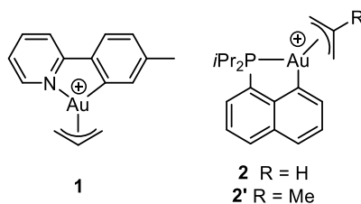
Figure 2. First \pi -allyl Au(III) complexes authenticated.
