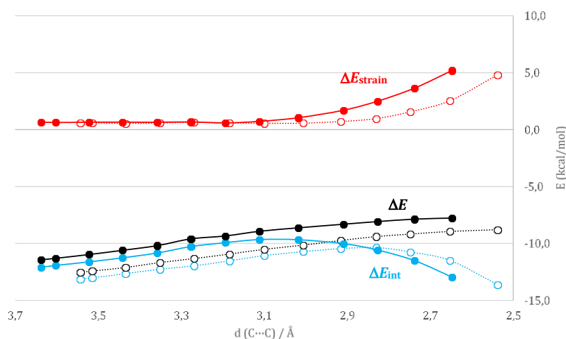
Figure 9. Comparison of the Activation Strain diagrams accounting for the nucleophilic attack of 3a at C_{\text{cent}} (dotted lines) and C_{\text{term}} cis to P (solid lines) of the \pi -allyl complex 2 computed at SMD(THF)-B3PW91/SDD+f(Au),6-31G**(other atoms) level of theory.
