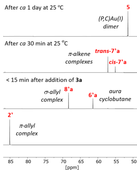
Figure 6. Stacked 31 P NMR spectra showing the progress of the reaction between the \pi -allyl Au(III) complex 2' and enolate 3a in d_8 -THF (Top: at 25 °C and 121.49 MHz, otherwise: at -20 °C and 202.45 MHz).
