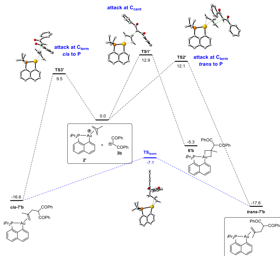
Figure 11. Energy profiles for the nucleophilic addition of enolate 3b to the \pi -methallyl Au(III) complex 2' computed at the SMD(THF)-B3PW91/SDD+f(Au),6-31G** (other atoms) level of theory. Gibbs free energies ( \Delta G ) in kcal/mol.
