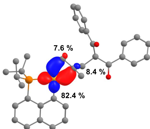
Figure 13. NLMO associated to d(\text{Au}) \rightarrow \pi^*(\text{C}=\text{C}) back-donation in the (P,C)-cyclometallated Au(I) \pi -complex trans-7b , with participation of main atoms in % (cutoff: 0.05). Hydrogen atoms have been omitted for clarity.
