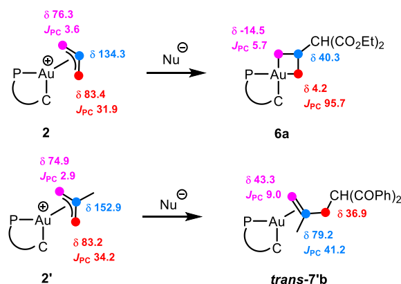
Figure 3. Diagnostic ^{13}\text{C} NMR resonances for the allyl fragment in the \pi -allyl complexes 2/2' , auracyclobutane 6a and \pi -alkene complex 7'b (data in d_8 -THF, chemical shifts in ppm, coupling constants in Hz).
