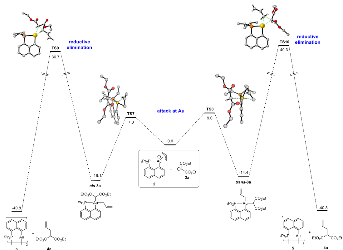
Figure 10. Alternative inner-sphere pathway for the reaction of enolate 3a with the \pi -allyl Au(III) complex 2 computed at SMD(THF)-B3PW91/SDD+f(Au),6-31G**(other atoms) level of theory. Gibbs free energies ( \Delta G ) in kcal/mol.
