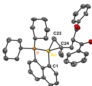
Figure 4. Molecular structure of the \pi -alkene Au(I) complex 7'b-Cy (hydrogen atoms omitted for clarity, ellipsoids shown at 50% probability). Selected bond lengths (Å) and angles (°): Au–C23 2.144(5), Au–C24 2.158(4), C23–C24 1.420(9), P–Au–C23 122.9(2), P–Au–C24 160.6(2), C1–Au–C23 152.6(2), C1–Au–C24 114.1(2), P–Au–C1 84.3(1).
