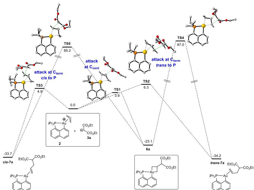
Figure 8. Energy profiles for the nucleophilic addition of enolate 3a to the \pi -allyl Au(III) complex 2 computed at the SMD(THF)-B3PW91/SDD+f(Au),6-31G**(other atoms) level of theory. Gibbs free energies ( \Delta G ) in kcal/mol.
