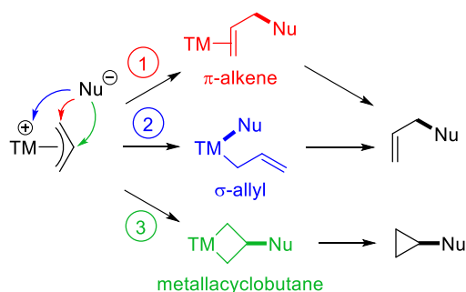
Figure 1. Possible reactive sites for the addition of nucleophiles to \pi -allyl complexes.
