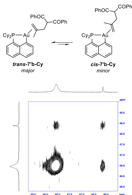
Figure 5. Trans and cis isomers of the \pi -alkene Au(I) complex 7'b-Cy and ^{31}\text{P} - ^{31}\text{P} EXSY spectrum (202.45 MHz, \text{CD}_2\text{Cl}_2 , -10^\circ\text{C} , mixing time 250 ms) substantiating their interconversion.
