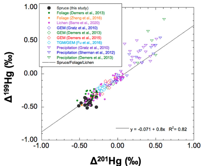
Fig. 5. \Delta^{201}\text{Hg} vs. \Delta^{199}\text{Hg} for spruce samples in this study compared with those for foliage, lichen, GEM, and precipitation samples in the literature.
