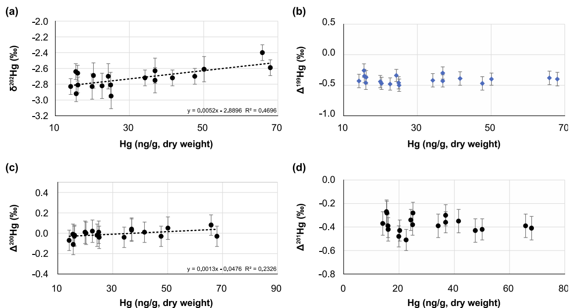
Fig. 3. Hg concentration vs. (a) \delta^{202}\text{Hg} , (b) \Delta^{199}\text{Hg} , (c) \Delta^{200}\text{Hg} , and (d) \Delta^{201}\text{Hg} in spruce. Uncertainties of each plot represent 2SD of NIST RM 8610 as reported in Table S3.
