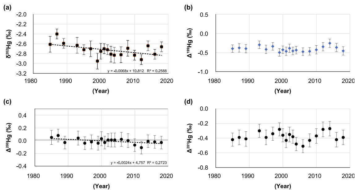
Fig. 2. Temporal variations of (a) \delta^{202}\text{Hg} , (b) \Delta^{199}\text{Hg} , (c) \Delta^{200}\text{Hg} , and (d) \Delta^{201}\text{Hg} in spruce. The uncertainties of each plot represent 2SD of NIST RM 8610 as reported in Table S3.
