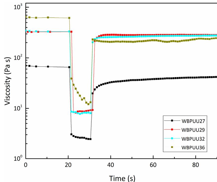
Figure 4. Structure recovery test of WBPUU based inks with different solid contents ( T = 22.5 \text{ }^{\circ}\text{C} ).
