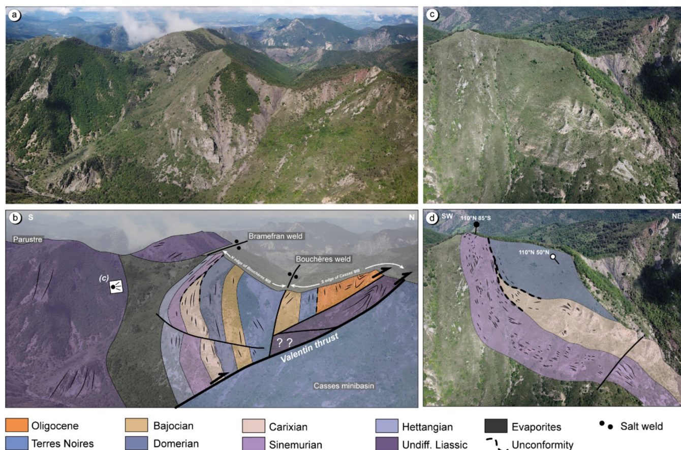
Fig. 17. (a) and (b) Uninterpreted and interpreted panorama of the Bramefran and Valentin highs, showing the Valentin thrust cutting through the Bouchères weld. (c) and (d) Uninterpreted and interpreted pictures of the pinch out of the Carixian near the Bramefran weld, see location of the picture on (b).
