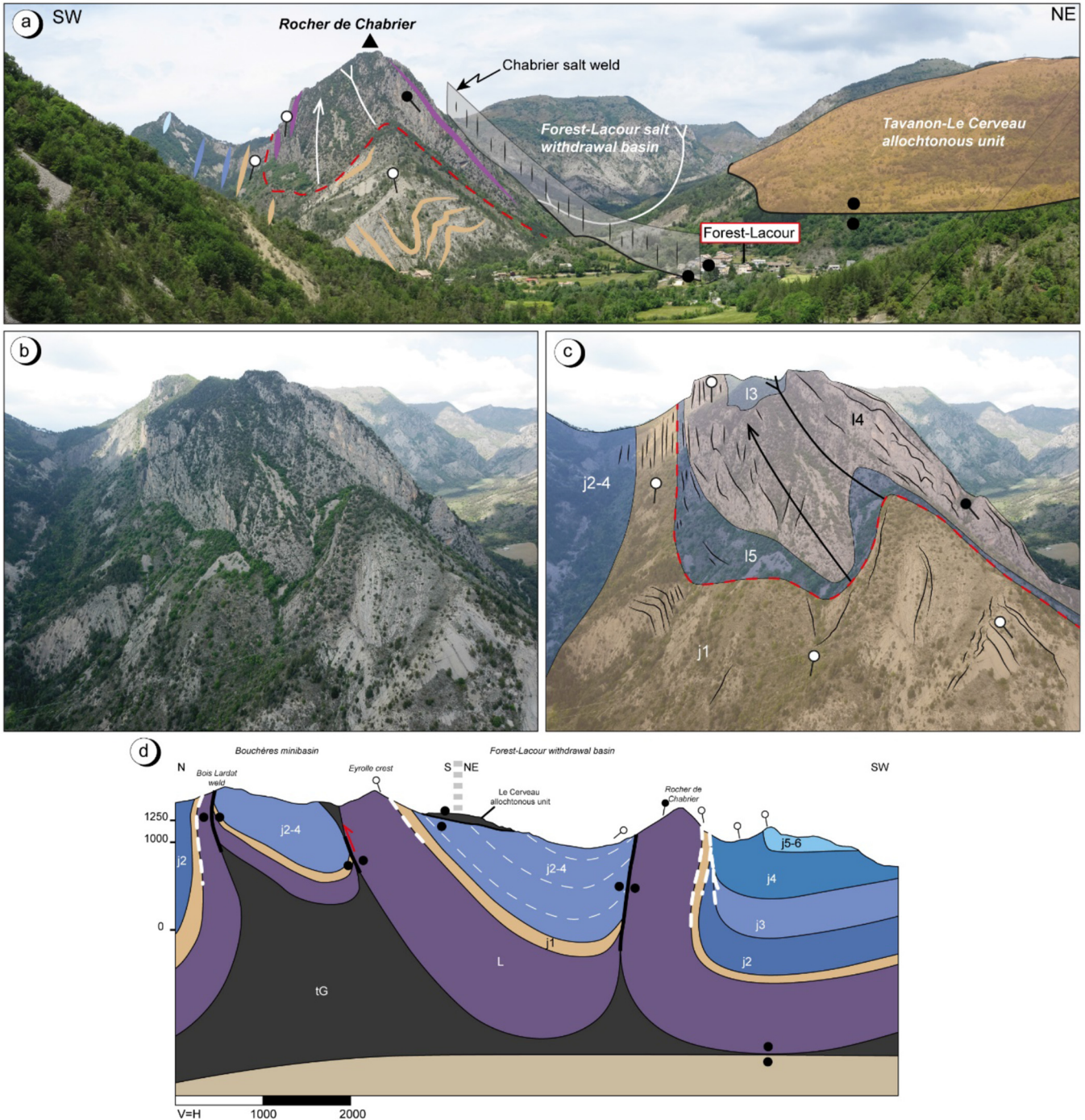
Fig. 12. (a) Interpreted panorama of the Rocher de Chabrier megaflap and the associated Forest-Lacour salt withdrawal basin (rim syncline) both on each side of the vanished Chabrier salt structure. (b) Zoom on the Rocher de Chabrier tight anticline and syncline illustrating the early deformation of the megaflap. (c) Interpreted picture of the Rocher de Chabrier zoom. (d) Interpretative cross-section through the Rocher de Chabrier and the Forest-Lacour rim syncline. See location of the cross-section in Figure 4 .
