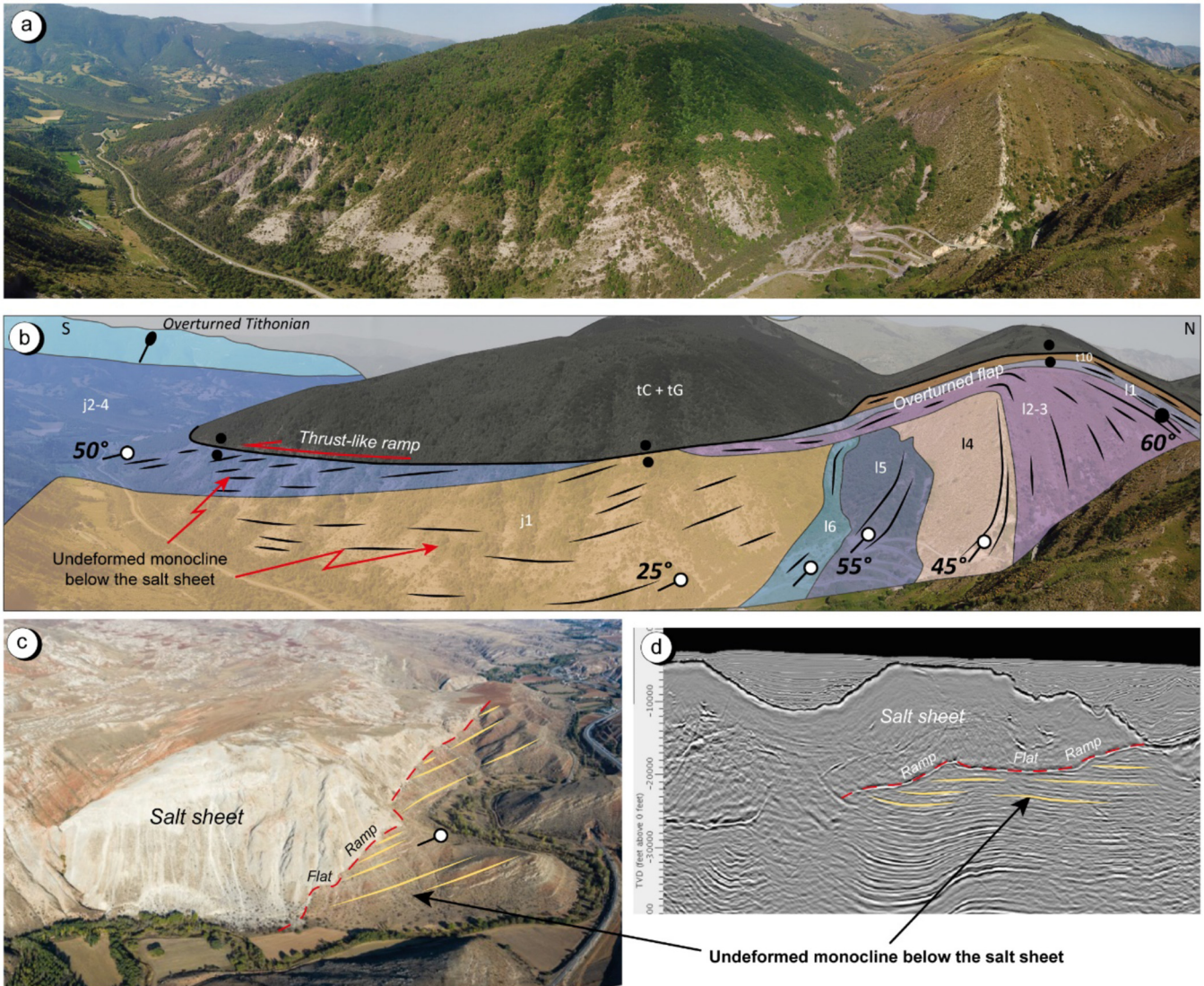
Fig. 15. (a) and (b) Uninterpreted and interpreted panoramas of the Astoin megaflap and its southern continuation which forms an allochthonous salt sheet during the Jurassic. (c) Analogue onshore salt sheet in the Sivas Basin in Turkey (picture from JC Ringenbach). (d) Analogue offshore salt sheet in seismic line in the Gulf of Mexico. The Astoin allochthonous salt sheet ((a) and (b)) presents the same features of salt sheets ((c) and (d)) which are: a contact which climbs upward into the stratigraphy between the allochthonous salt and its substratum and the undeformed monocline of the substratum below the salt sheet.
