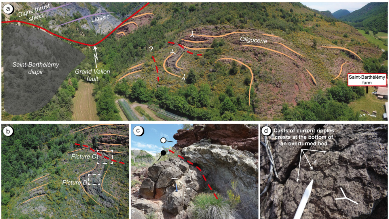
Fig. 9. (a) Photo of the Oligocene strata near the Saint-Barthélémy farm showing the global pattern of the Oligocene which is twice overturned below younger Oligocene, forming two successive hook halokinetic sequences. (b) Zoom on one hook halokinetic sequence showing Oligocene overturned strata below younger Oligocene strata and the unconformity between. (c) Zoom on the unconformity. (d) Picture of casts of the crest of current ripples marks at the bottom of a bed, testifying that the Oligocene is overturned.
