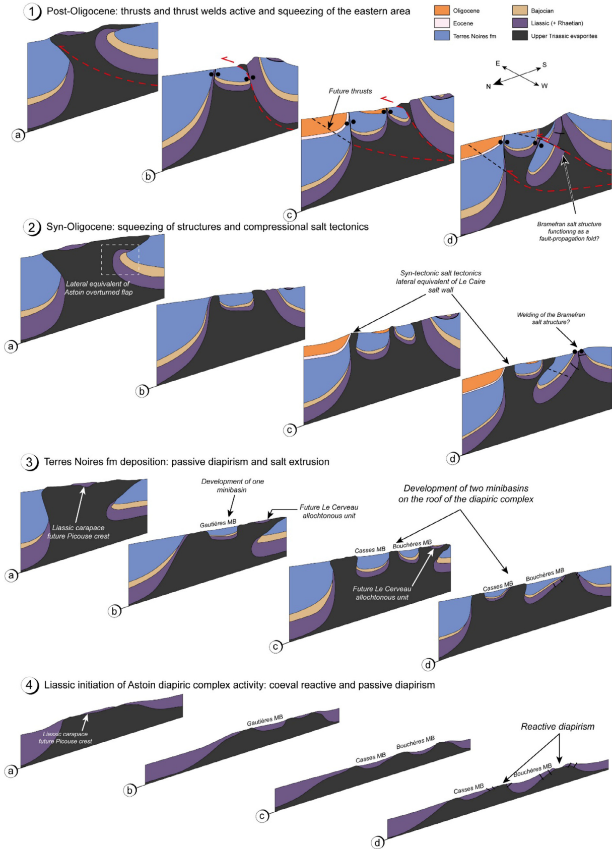
Fig. 19. Time step reconstruction of the cross-sections through the Picouse–Valentin sector, present-day cross-sections in Figure 18 .
