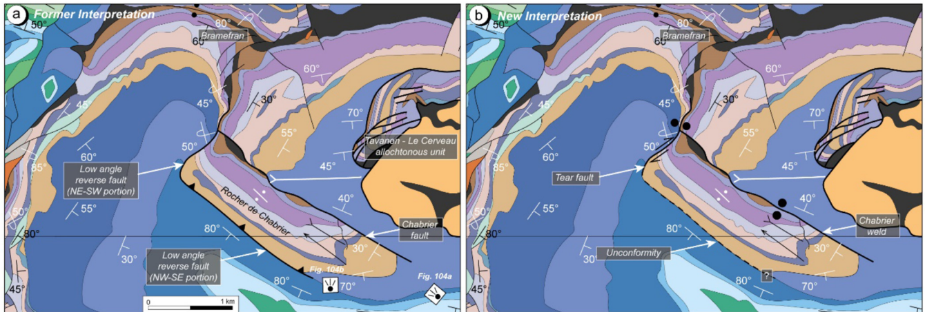
Fig. 11. Zoom on the geological map of Figure 3, focused on the Rocher de Chabrier.
