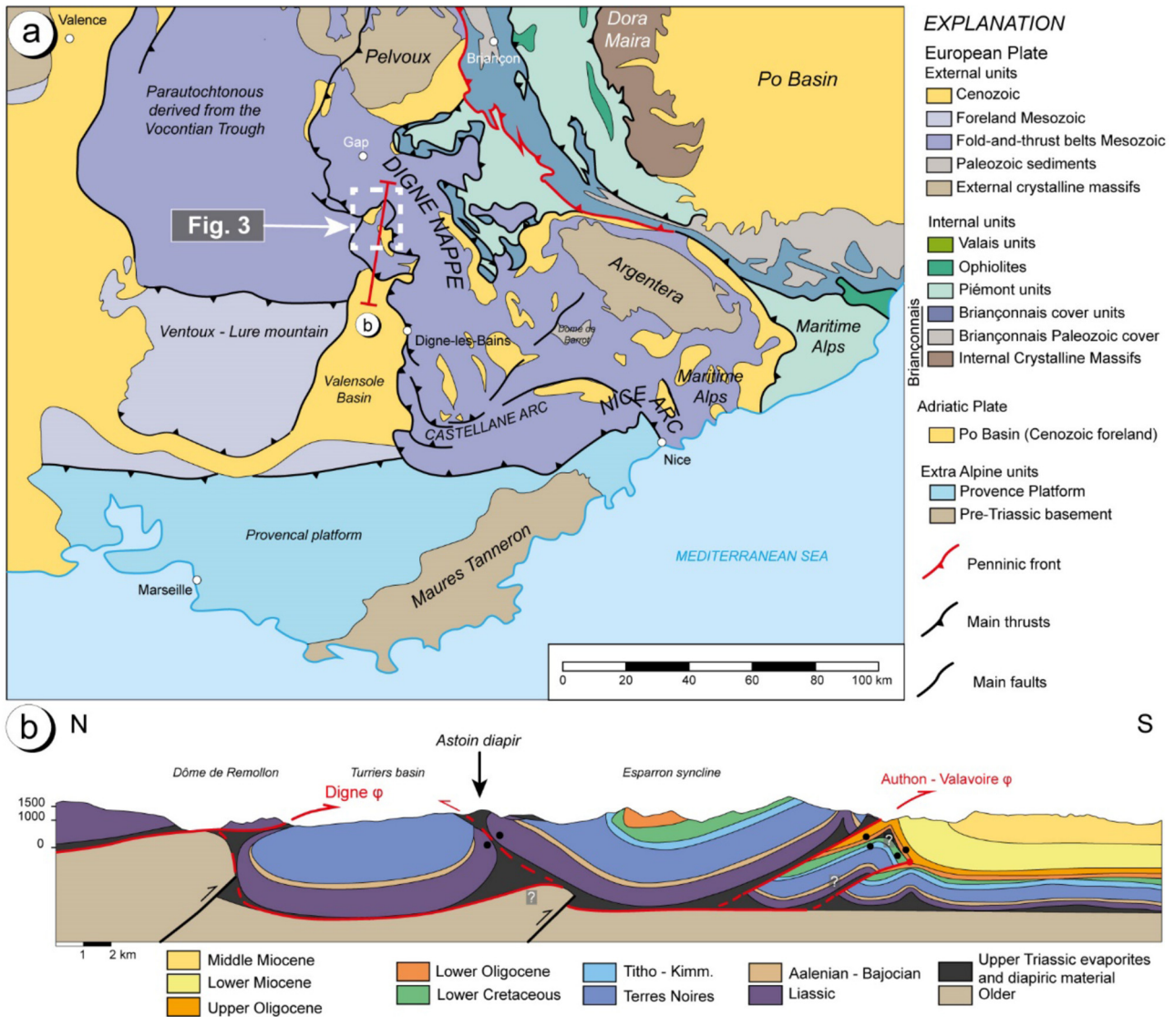
Fig. 1. (a) Structural sketch from SE France modified from Pffner (2014). (b) Cross-section of the Digne Nappe near the Astoin diapir (Célini et al. , 2020).
