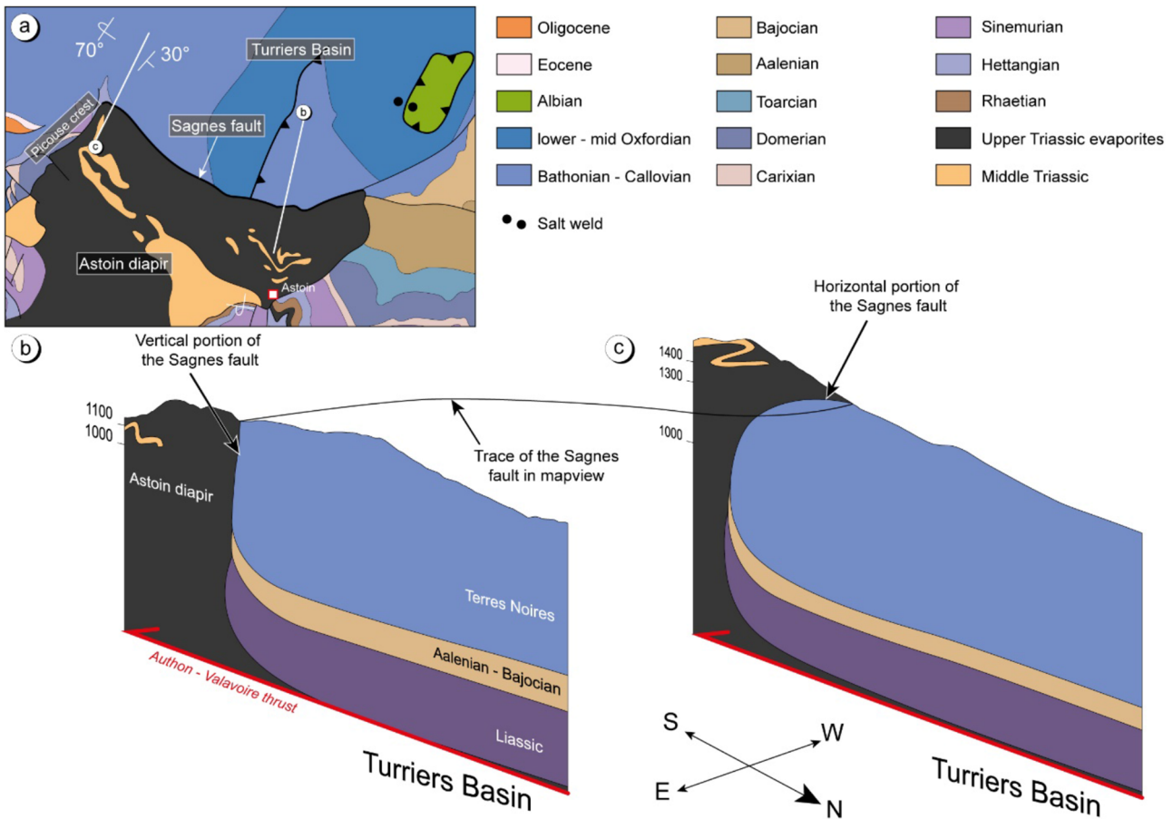
Fig. 6. (a) Zoom of the geological map on the Astoin diapir and the southern termination of the Turriers basin. (b) Interpretative cross-section through the Sagnes fault in the eastern part of the diapir. (c) Interpretative cross-section through the Sagnes fault in the western part of the diapir.
