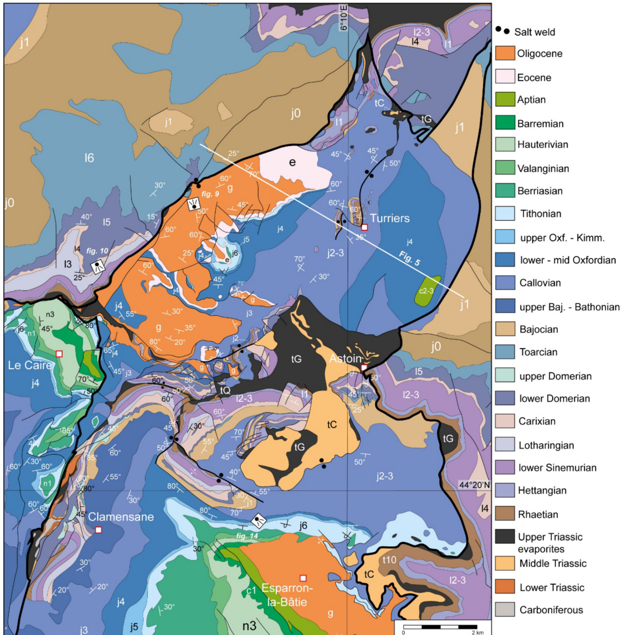
Fig. 3. Geological map of the study area modified and harmonised after the geological maps of France at 1/50 000 from the BRGM.
