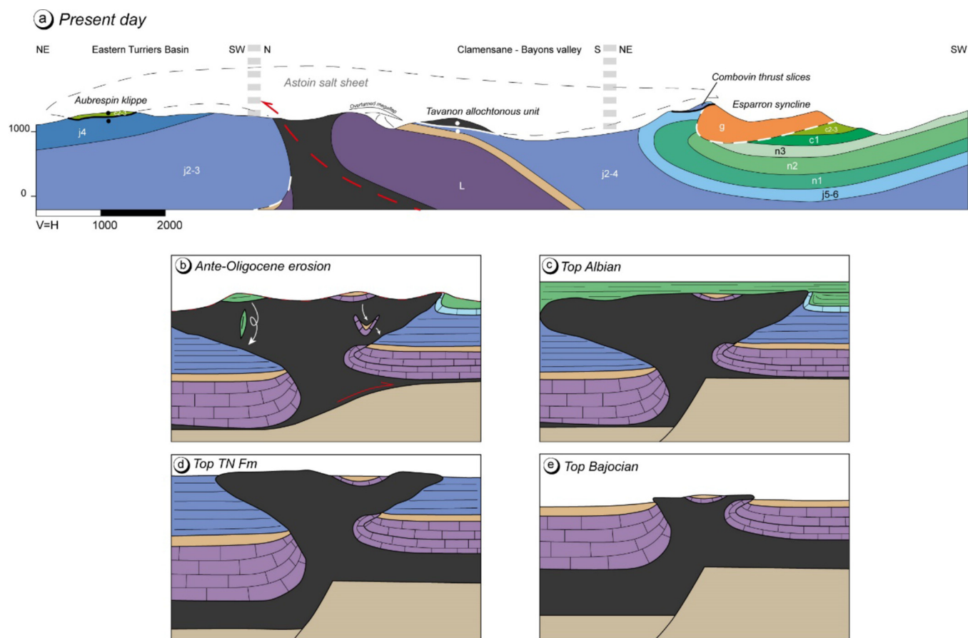
Fig. 16. Present-day interpretative cross-section illustrating the Astoin allochthonous salt sheet inherited from the passive margin stage preserved into an orogen. See location of the cross-section in Figure 4 . (b), (c), (d) and (e) are simplified sketches illustrating the emplacement of the allochthonous salt sheet.
