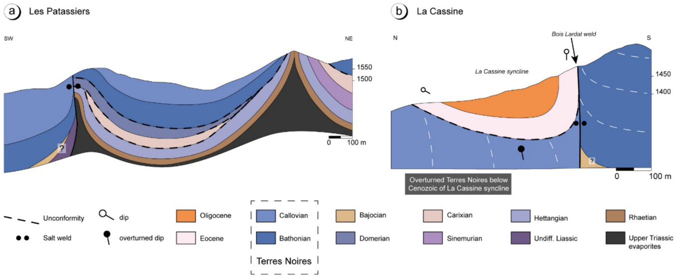
Fig. 8. (a) Interpretative cross-section through the Les Patassiers structure. (b) Cross-section through the Bois Lardat weld and the La Cassine syncline. See location of cross-sections in Figure 7.
