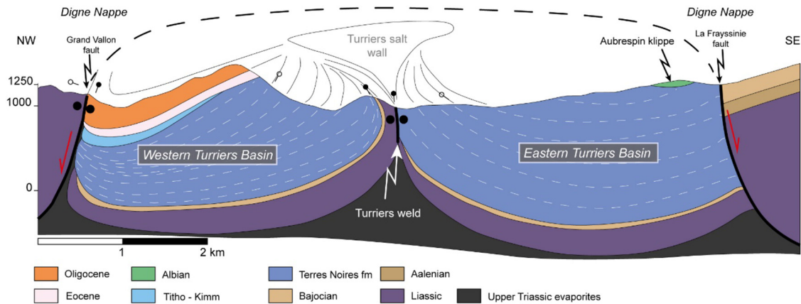
Fig. 5. Cross-section through the Turriers basin, modified from Célini et al. (2020). See location of the cross-section in Figure 3.
