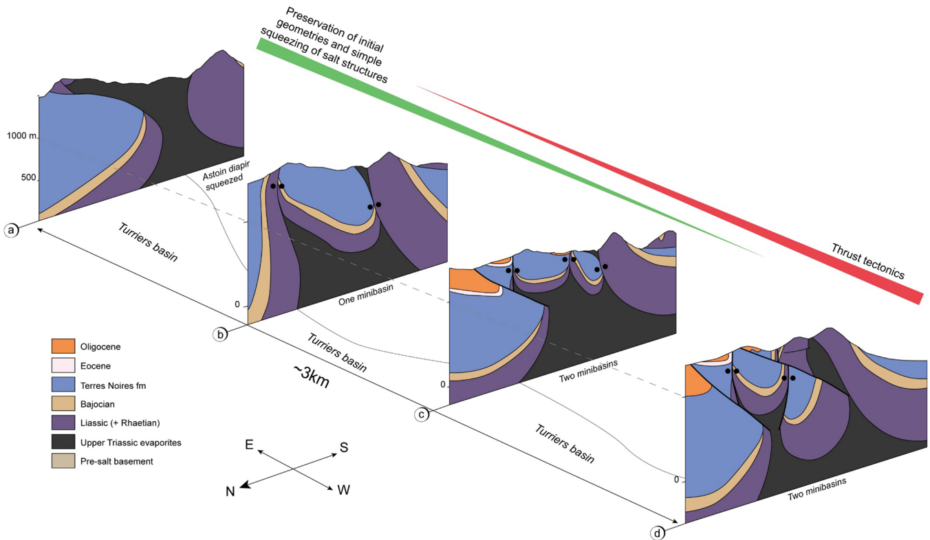
Fig. 18. Serial interpretative cross-sections through the Picouse–Valentin sector. See locations of cross-sections in Figure 7b .
