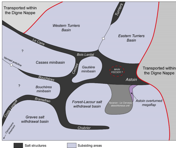
Fig. 20. Map view of the Astoin diapiric complex with the salt structures and the associated rim synclines in their palinspastic position during the Jurassic. The schema is not to scale and its aim is to locate the different structures in their original position.
