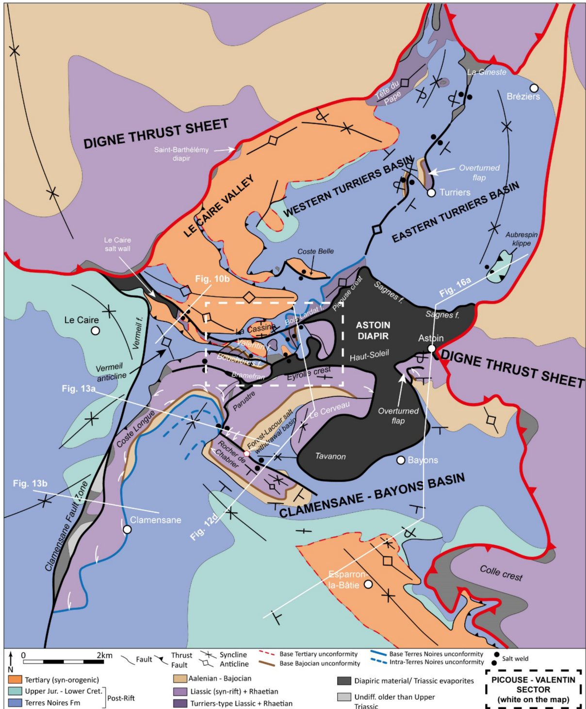
Fig. 4. Structural sketch of the study area with the main locations.
