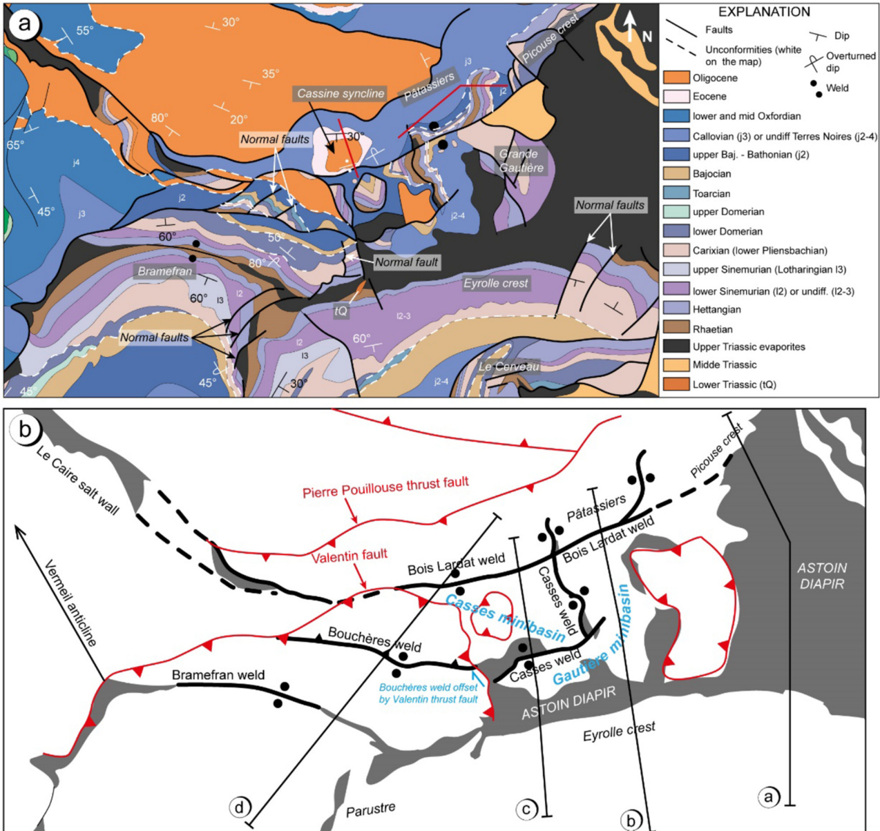
Fig. 7. (a) Geological map of the Picouse–Valentin sector (See location in Fig. 4). (b) Structural sketch of the Picouse–Valentin sector with the main structural relationships (faults and welds). Black lines correspond to the locations of cross-sections in Figure 18.
