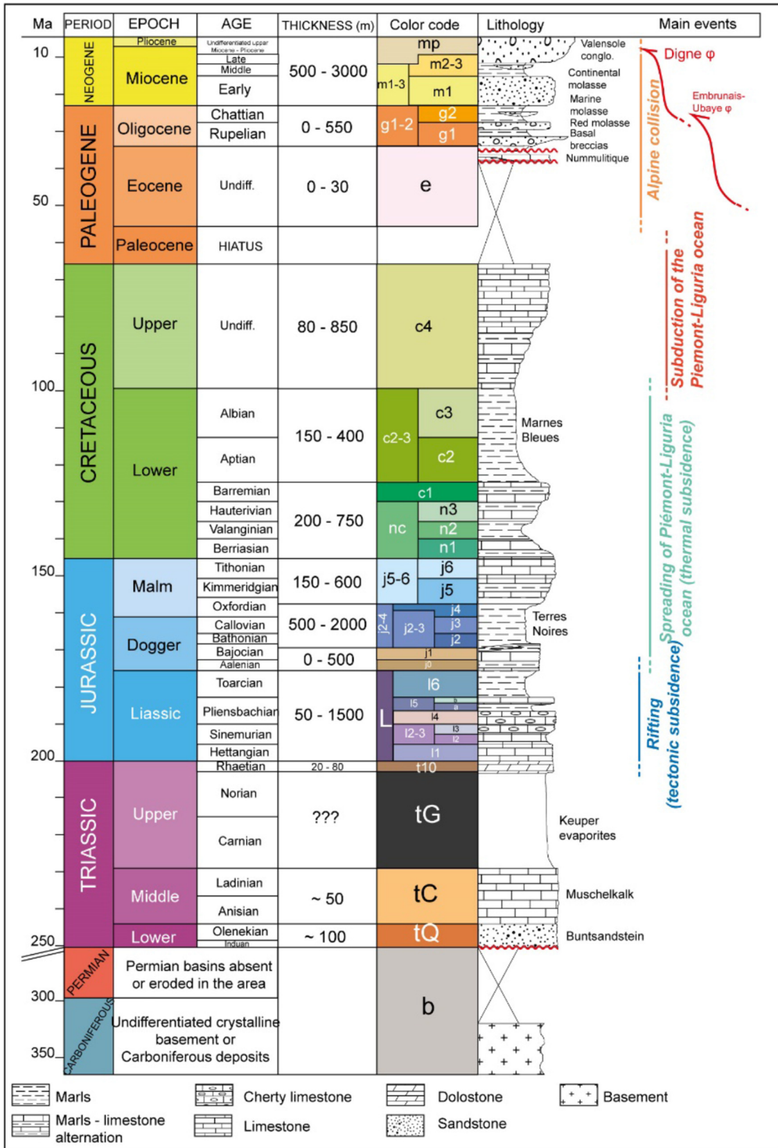
Fig. 2. Stratigraphy of the Astoin diapir area.
