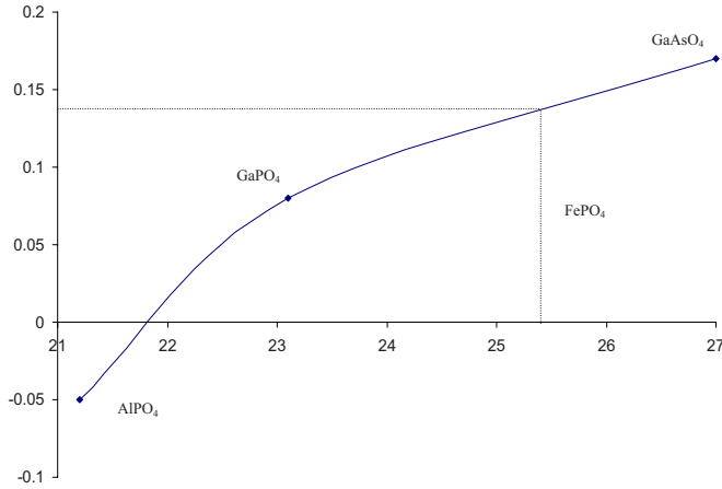
FIG. 4. (Color online) Piezoelectric constant e_{14} (in \text{C}/\text{m}^2 ) as a function of the tilt angle \delta (in degrees).
