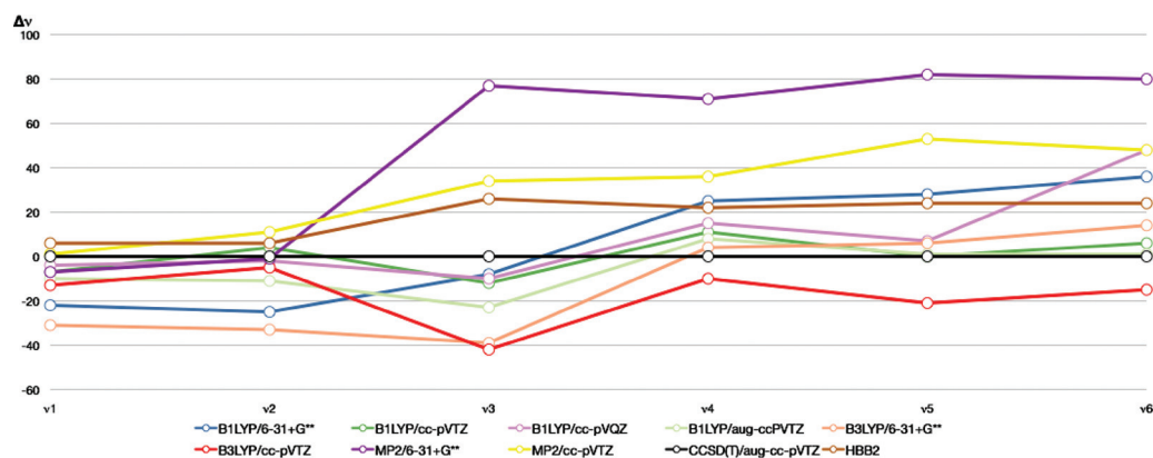
FIG. 3. (3n-6)-k calculated harmonic frequencies of the water (\text{H}_2\text{O})_{n=2} dimer (k torsional modes). The color lines relate to the difference between the CCSD(t)/avtZ harmonic frequencies (Ref. 62) (black circle) and other levels of theories.
