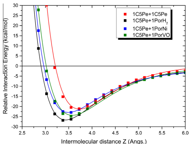
Fig. 6. Attraction-repulsion curves for the C5Pe-C5Pe, C5Pe-PorH 2 , C5Pe-PorNi, and C5Pe-PorVO in S 0 state (D 0 for C5Pe-PorVO) calculated within the DFT level of theory.
