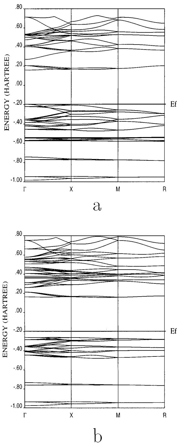
FIG. 1. HF band structures of the \alpha (a) and \beta (b) states at the experimental geometry.
