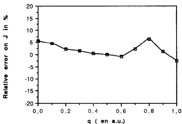
Fig. 5. Relative difference percentage between calculated and experimental valence Compton profile for the low energy side of polycrystalline \text{MgH}_2 .
