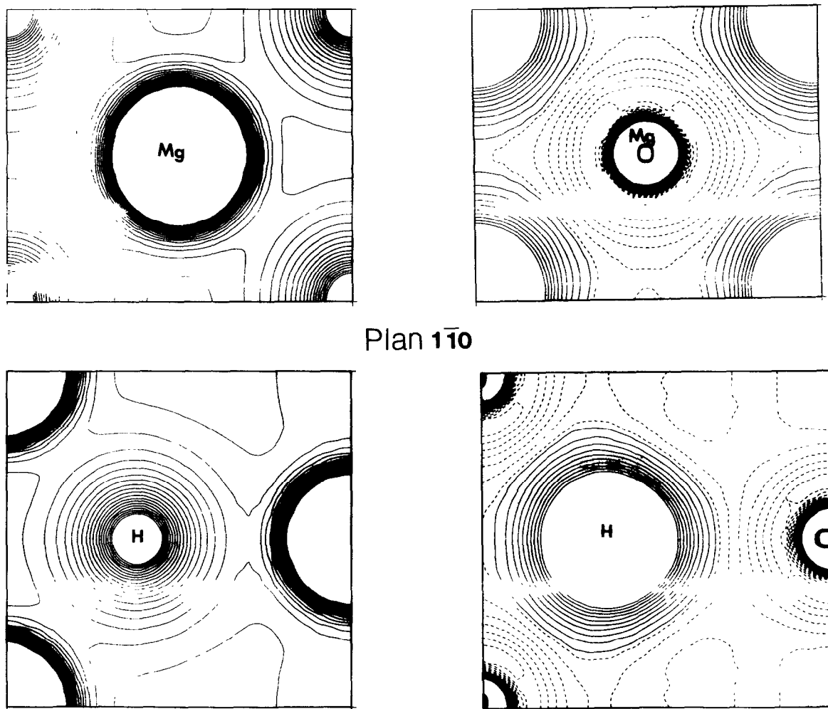
Fig. 4. Total and difference (crystal minus ionic superposition) electron density map on the (110) and (1\bar{1}0) planes. Isodensity curves are separated by 0.01 \text{ e/bohr}^3 and by 0.001 \text{ e/bohr}^3 for total and difference charge density respectively. Continuous and dashed lines indicate positive and negative values, respectively.
