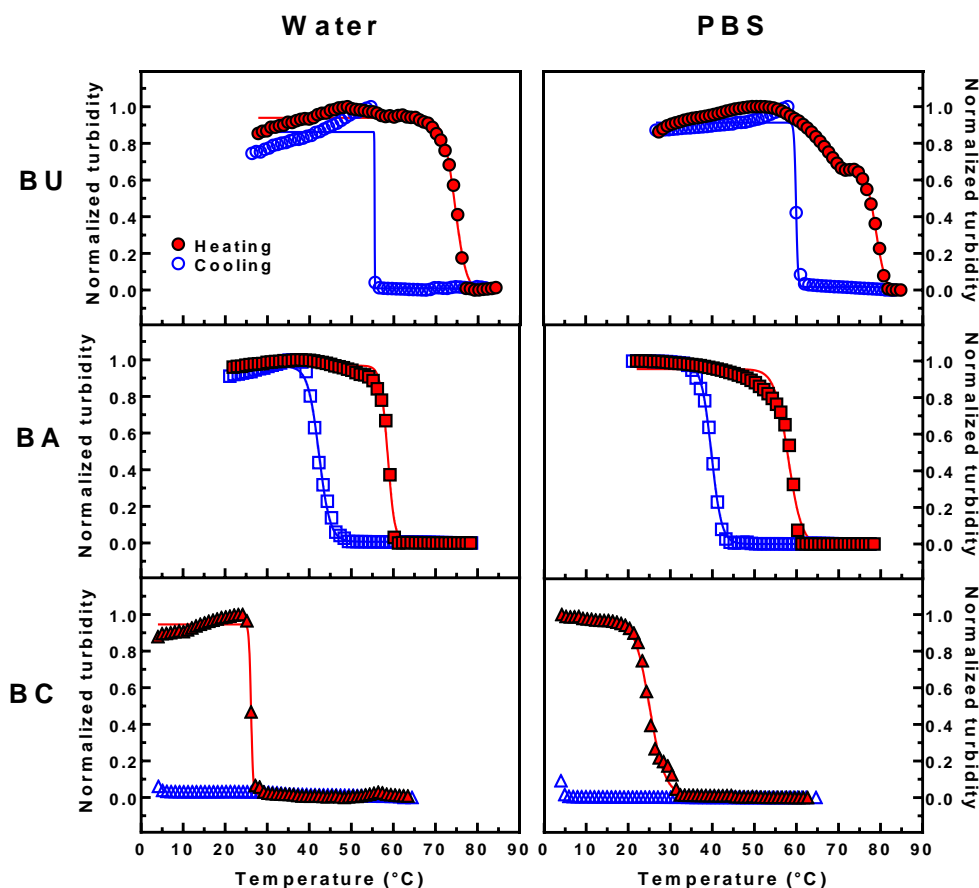
Figure 7. Turbidimetry of BU (top), BA (middle), BC (bottom) during heating (red full symbols) and cooling cycles (blue open symbols) in water (left) or PBS (right). Condition: [GNB] = 1% w/v. Temperature ramp: 1\text{ }^{\circ}\text{C min}^{-1} .
