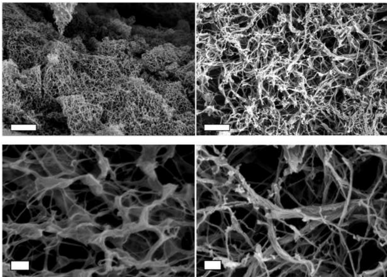
Figure 2. Scanning cryo-electron micrographs. BU (left panels) and BA (right panels) at two magnifications, scale bar = 1 \mu\text{m} (top panels) or 200nm (bottom panels). Condition: 1% w/v prepared in PBS.
