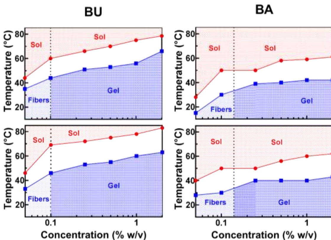
Figure 14. Phase diagrams. T_m and the T_c function of concentration of BU (left panels) or BA (right panels) in water (top panels) or in PBS (bottom panels). Vertical dashed plot corresponds to the critical gelation concentration (CGC). Red line separating the sol phase part and blue line separating the self-assembled part correspond to the T_m and the T_c , respectively. The white part of the diagrams represents the hysteresis.
