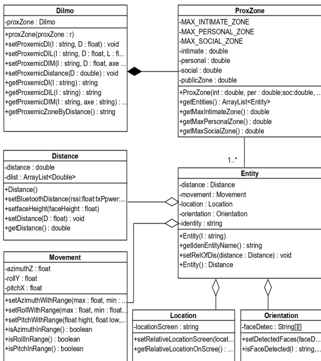
Figure 3. UML Class Diagram of the API.
