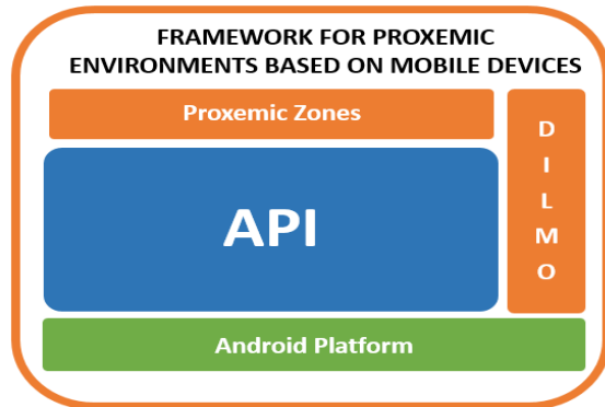
Figure 1. Framework architecture.
