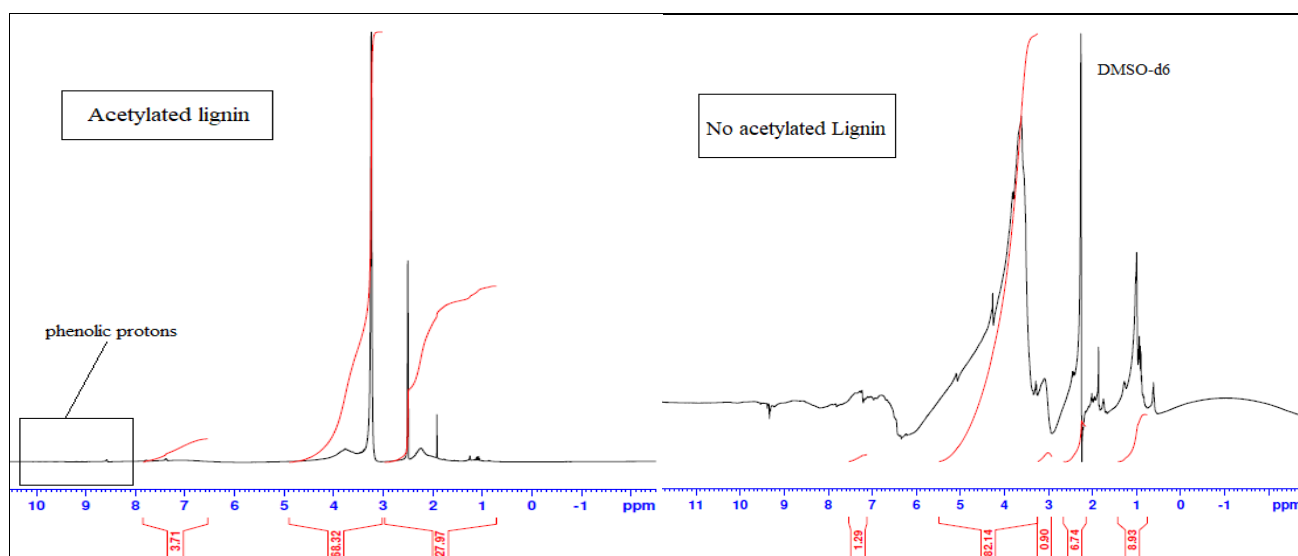
Figure 5. ^1\text{H} -NMR spectrum of acetylated lignin and lignin original
