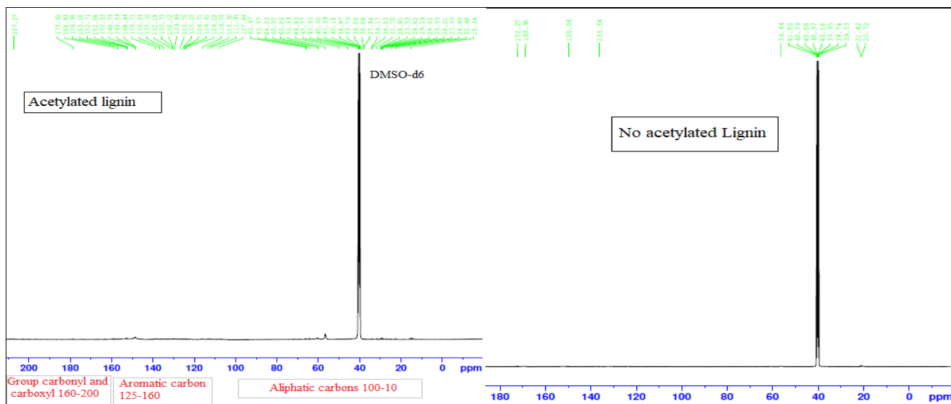
Figure 4. ^{13}\text{C} -NMR spectrum of acetylated lignin and lignin original
