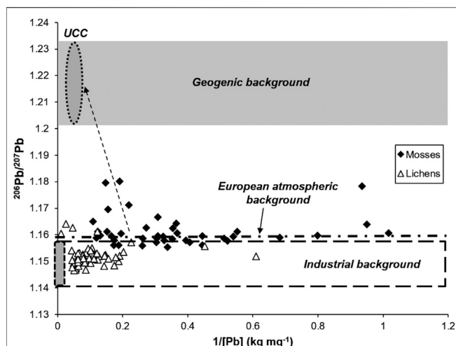
FIGURE 2 | ^{206}\text{Pb}/^{207}\text{Pb} vs. 1/[\text{Pb}] in \text{kg}/\text{mg} diagram for lichens and mosses. Upper continental crust (UCC) data issued from Millot et al. (2004), Wedepohl (1995) et Weiss et al. (1999). Industrial data are from Geagea et al. (2008), Monna et al. (1997) and Cloquet et al. (2006).
