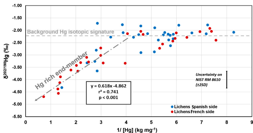
FIGURE 6 | \delta^{202/198}\text{Hg} vs. 1/[\text{Hg}] for lichens from Iraty Forest. Blue dots correspond to lichens of the Spanish sampling sites while red dots correspond to lichens of the French sampling sites. The trend suggests a contamination end member of about -4.86 \pm 0.21\% ( p < 0.001 ) for 1/[\text{Hg}] = 0 .
