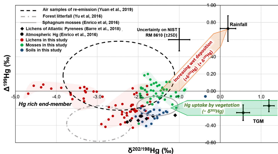
FIGURE 5 | Tri-isotopic plot of \Delta^{199}\text{Hg} vs. \delta^{202/198}\text{Hg} (‰) for lichens, mosses and soils from Iraty forest. Uncertainties are expressed for the long-term reproducibility of NIST RM 8610 (former UM-Almadén) (as 2 SD) by CVG.
