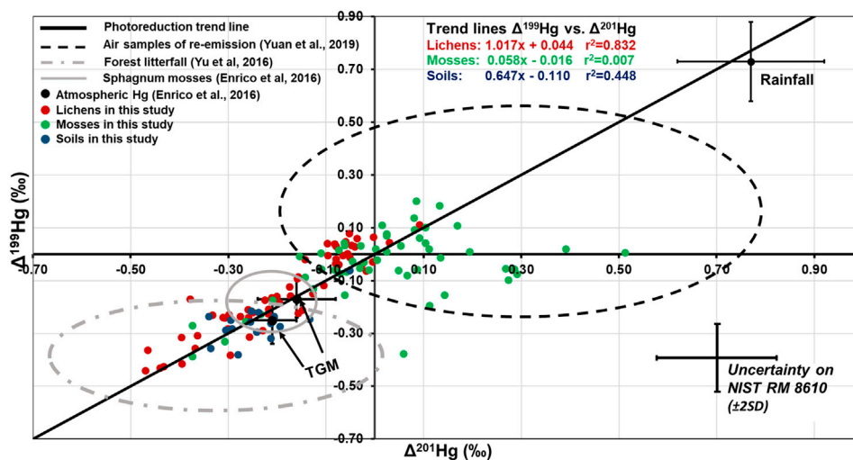
FIGURE 4 | \Delta^{199}\text{Hg} vs. \Delta^{201}\text{Hg} in lichens, mosses and soils. Uncertainty calculated for NIST RM 8610 (former UM-Almadén) (as 2 SD) represents the long-term reproducibility of the method for CVG. \text{Hg}^{2+} photoreduction line is from Bergquist and Blum, 2009.
