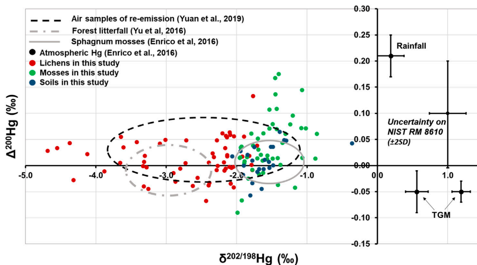
FIGURE 3 | \Delta^{200}\text{Hg} vs. \delta^{202/198}\text{Hg} in lichens, mosses and soils. Uncertainty calculated for BCR 482 represent the reproducibility of the NIST RM 8610 (former UM-Almadén) (as 2 SD). The data were compared with other data from bibliography.
