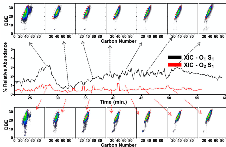
Figure 7. Extracted ion chromatograms and plots of DBE vs carbon number shown in order of elution from left to right for the O 1 S 1 (top) and O 2 S 1 (bottom) heteroatom classes from the PetroPhase 2017 asphaltenes.
