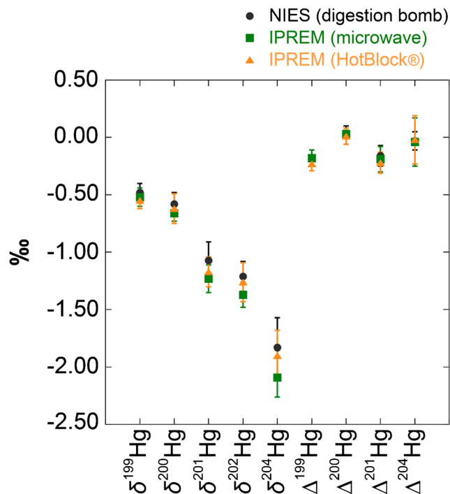
Fig. 1 Hg isotopic compositions of NIES CRM No. 28. Three digestion methods were implemented in this study (digestion bomb: black circle; microwave: green square; and HotBlock®: orange triangle). The error bars on the CRM represent 2SD of Hg isotope heterogeneity from Table 5. IPREM, Institut Pluridisciplinaire de Recherche sur l'Environnement et les Matériaux; NIES, National Institute for Environmental Studies
