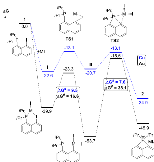
Figure 7. Overlay of the energy profiles computed for the reactions of the peri -iodo naphthyl phosphine 1-I with CuI and AuI at the SMD(DCM) B3PW91/SDD+f(M),SDD(I),6-31G** (other atoms) level of theory. Free energies in kcal/mol.
