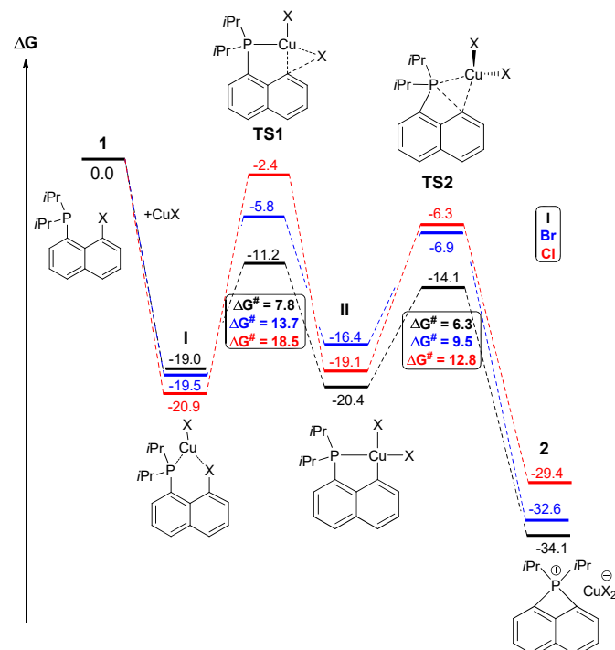
Figure 5. Energy profiles computed for the C–X oxidative addition (X: I, Br, Cl) / P–C reductive elimination sequence at the SMD(MeCN)-B3PW91/SDD+f(M),SDD(I,Br,Cl),6-31G**(other atoms) level of theory. Free energies in kcal/mol.
