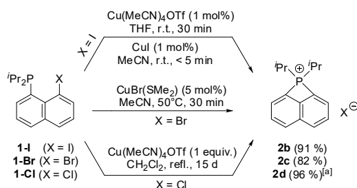
Scheme 5. Optimized conditions for the Cu-mediated transformation of peri -halogenated naphthyl phosphines 1-X into the corresponding peri -bridged naphthyl-phosphoniums 2b-d . [a] Yield based on 31 P NMR spectroscopy.
