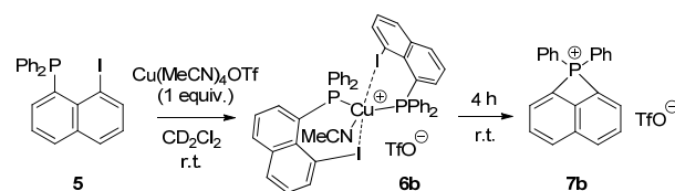
Scheme 4. Reaction of the diphenyl-substituted peri -iodo naphthyl phosphine 5 with \text{Cu}(\text{MeCN})_4\text{OTf} .
