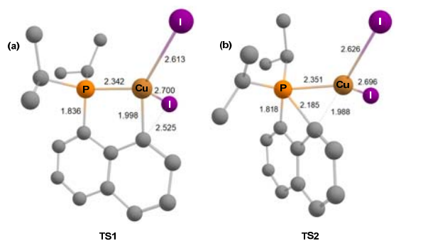
Figure 4. Transition states TS1 and TS2 computed respectively for the C–I oxidative addition (a) and P–C reductive elimination (b) at the SMD(DCM)-B3PW91/SDD+f(Cu),SDD(I),6-31G**(other atoms) level of theory. Key distances in Å.
