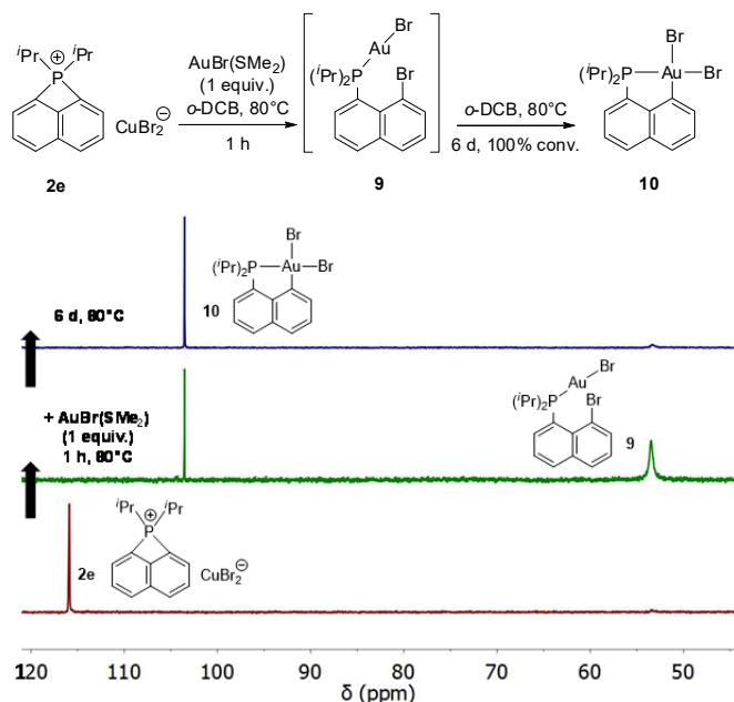
Scheme 7. Reaction of the peri -bridged phosphonium 2e with \text{AuBr}(\text{SMe}_2) leading to the (P,C)-cyclometallated dibromo gold(III) complex 10 . Below: ^{31}\text{P} NMR spectroscopic monitoring.
