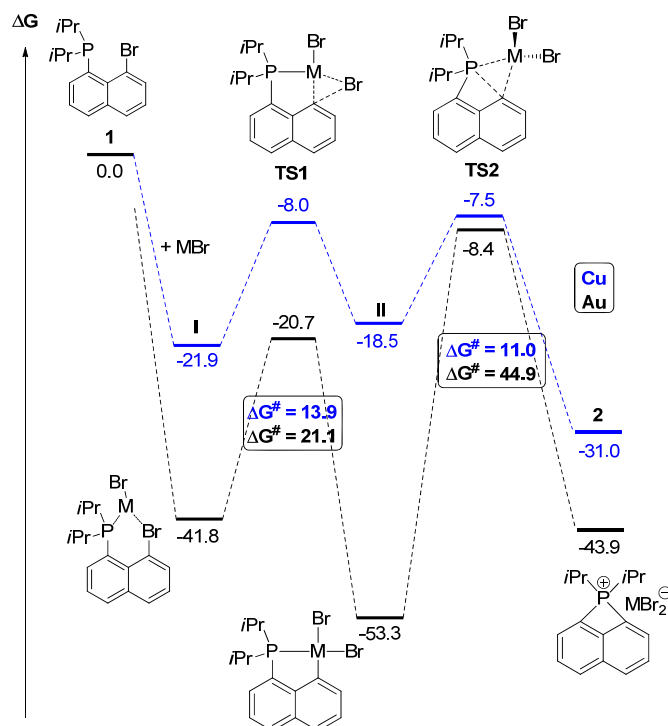
Figure 8. Overlay of the energy profiles computed for the reaction of the peri -bromo naphthyl phosphine 1-Br with CuBr and AuBr at the SMD(DCM)-B3PW91/SDD+f(M),SDD(Br),6-31G** (other atoms) level of theory. Free energies in kcal/mol.
