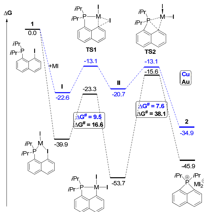
Figure 7. Energy profiles computed for the reactions of the peri -iodo naphthyl phosphine 1-I with CuI and AuI at the SMD(DCM) B3PW91/SDD+f(M),SDD(I),6-31G**(other atoms) level of theory. Free energies in kcal/mol.
