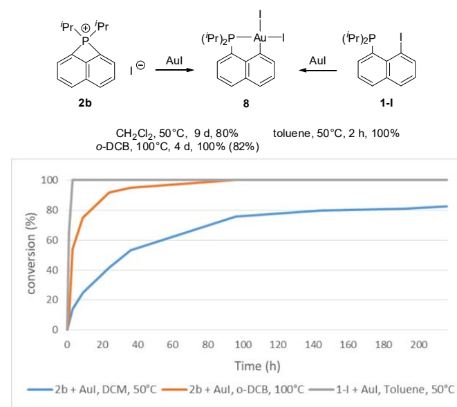
Scheme 6. Reactions of the peri -bridged naphthyl phosphonium 2b with AuI (isolated yield in parentheses) and alternative synthesis of the ensuing (P,C)AuI 2 complex 8 from 1-I . Below: graph showing the rates of conversion of 2b/1-I as determined by 31 P NMR spectroscopy.
