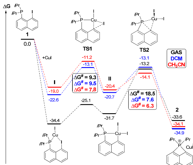
Figure 3. Energy profiles computed in the gas phase and in DCM/MeCN solutions for the C–I oxidative addition / P–C reductive elimination sequence. Free energies in kcal/mol computed at GAS-B3PW91/SDD+f(Cu),SDD(I),6-31G**(other atoms) and SMD(DCM or MeCN)-B3PW91/SDD+f(Cu),SDD(I),6-31G**(other atoms) levels of theory.
