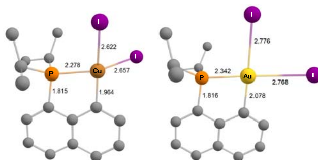
Figure 8. Structures computed for the (P,C)-cyclometallated M(III) complexes II (M = Cu, Au) at the SMD(DCM)-B3PW91/SDD+f(Cu),SDD(I),6-31G**(other atoms) level of theory. Key distances in Å.
