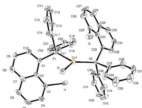
Scheme 3. Reaction of the diphenyl-substituted peri -iodo naphthyl phosphine 5 with \text{CuI} and crystallographic structure of the ensuing bis-phosphine \text{CuI} complex 6a .
