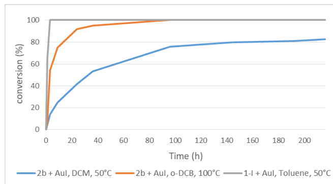
Scheme 6. Reactions of the peri -bridged naphthyl phosphonium 2b with AuI (isolated yield in parentheses) and alternative synthesis of the ensuing (P,C)AuI 2 complex 8 from 1-I . Below: graph showing the rates of conversion of 2b/1-I as determined by 31 P NMR spectroscopy.
