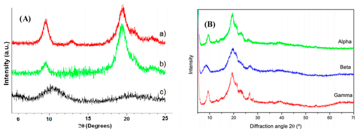
Figure 4. (A) XRD spectra of (a) chitin flakes, (b) chitin nanofibrils (CNF) and (c) a chitosan nanoparticles and chitosan nanofibers mixture [49]; and (B) X-ray diffractograms \alpha , \beta and \gamma -chitin [50].
