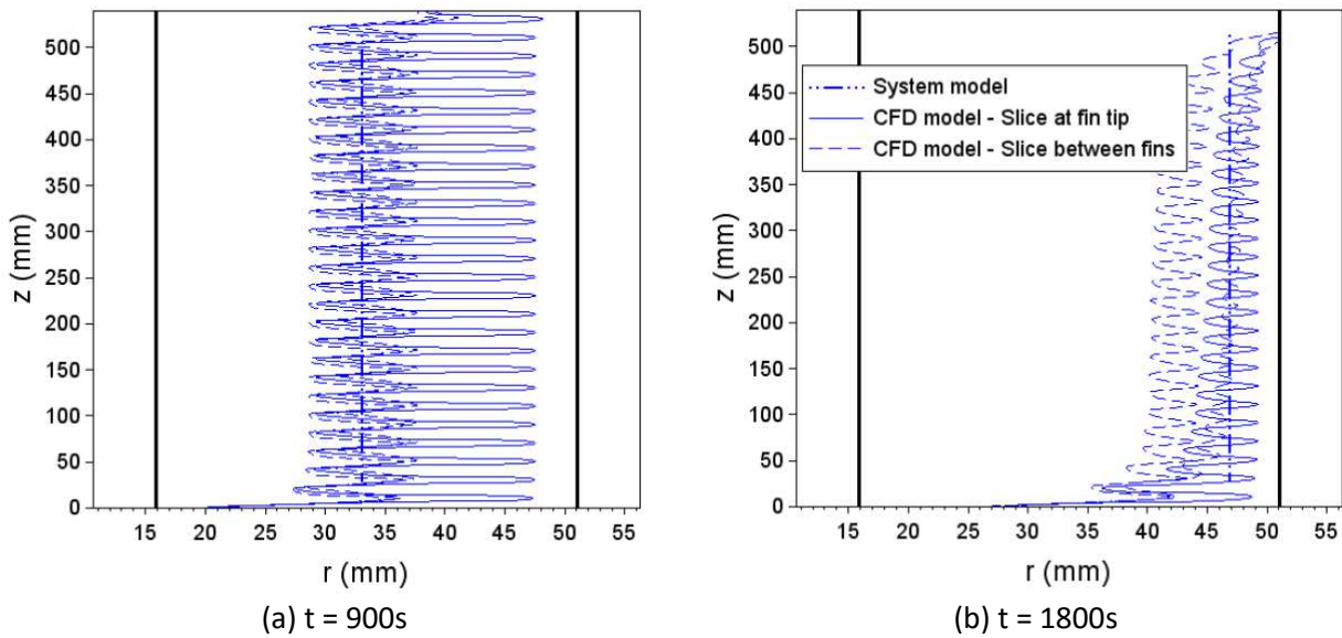
Figure 14: Comparisons of the phase fronts predicted by the CFD and system models for T_w = 328^\circ\text{C} (black lines represent the boundaries of the PCM domain. Left: outer tube wall. Right: external domain boundary.)
