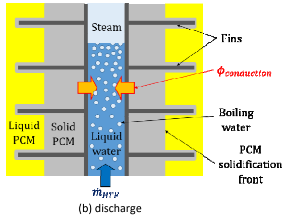
Figure 2 : Schematic view of the physical phenomena occurring in a shell-and-tube steam storage system based on LHS
