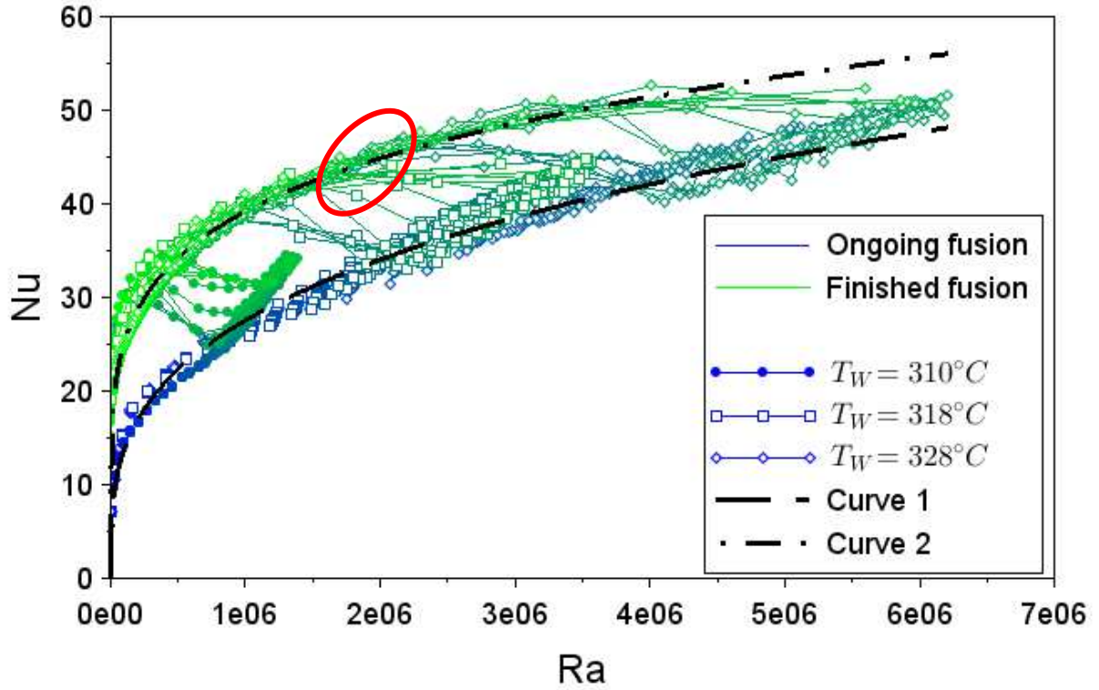
Figure 9: Comparisons of the (Ra, Nu) scatter plot obtained from the CFD results, using Eqs. (11) and (15) for the definitions of l_c and T_{PCM} , with correlations (16) and (17) for the heat transfer
