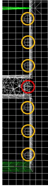
Figure 6: Mesh cells near the outer wall of the inner tube (yellow: PCM cells; red: fin cells)
