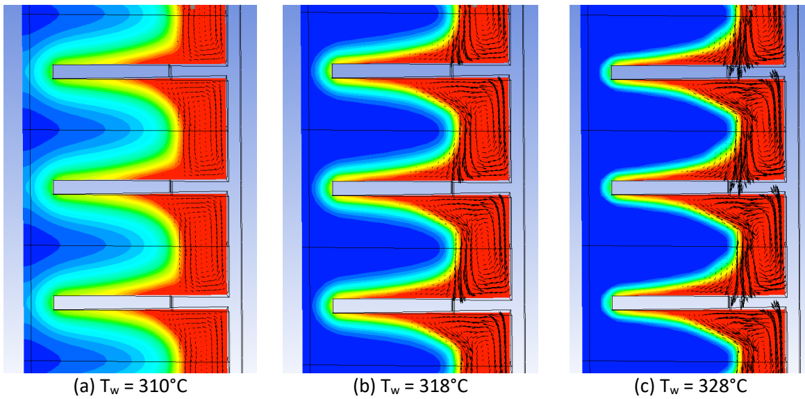
Figure 13: Liquid fraction and velocity fields in a vertical plane for the three CFD computations
