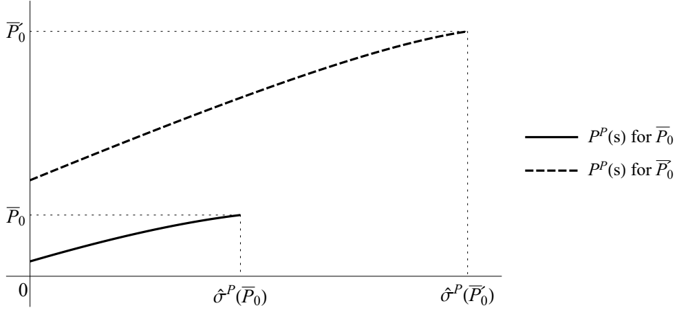
Figure 4: The equilibrium bidding strategy P^P(s) for two values of \bar{P}_0 .
