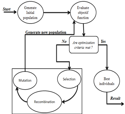
Figure 1. The Principle of the genetic algorithm.
