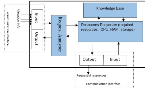
Figure 3. Analyzer Agent Architecture.
