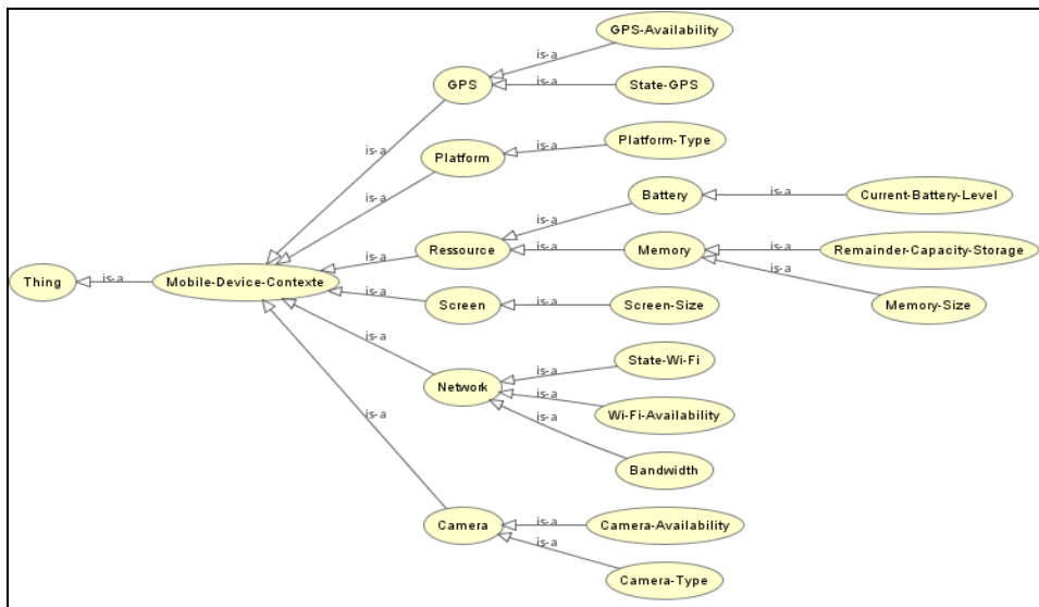
Fig. 1. Mobile device context ontology.
