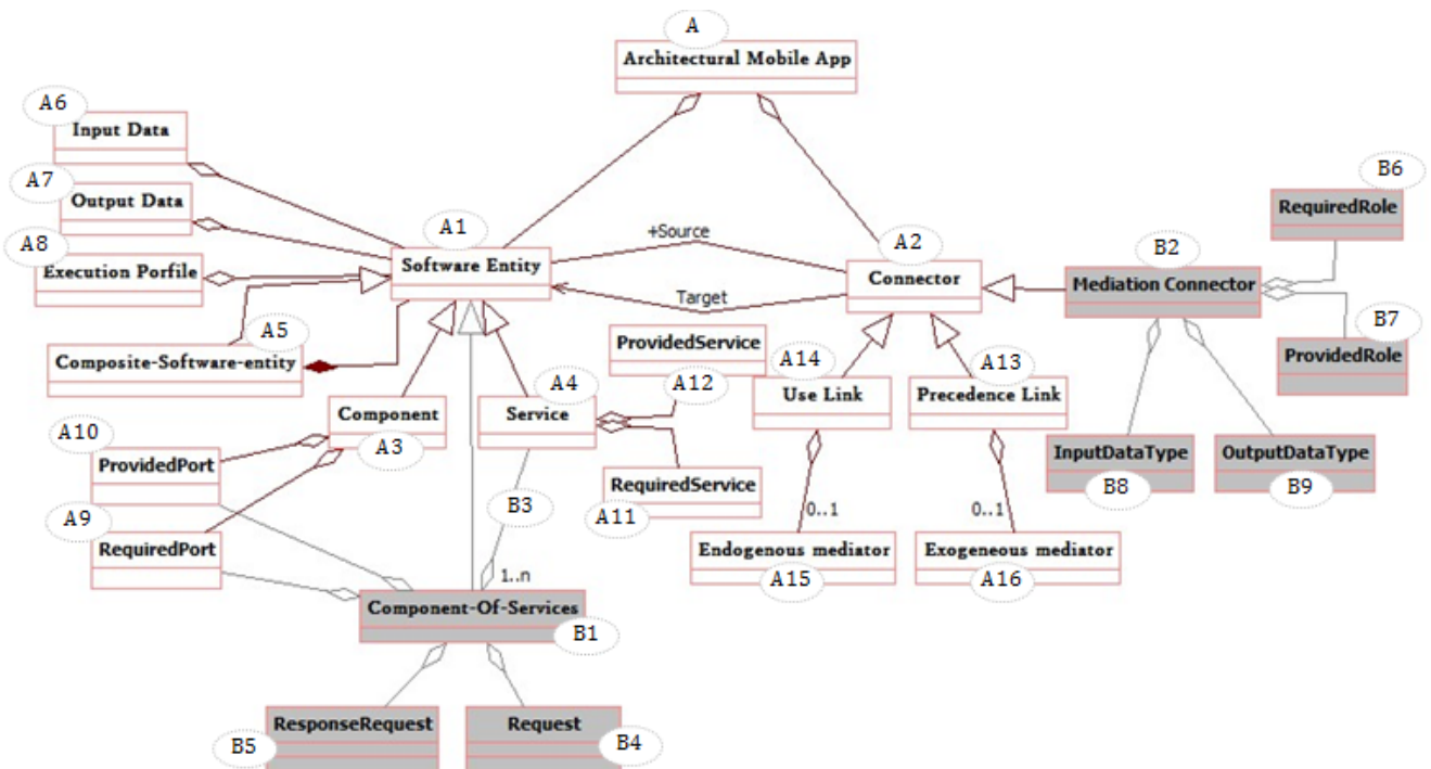
Figure 1 HMA-AD metamodel
