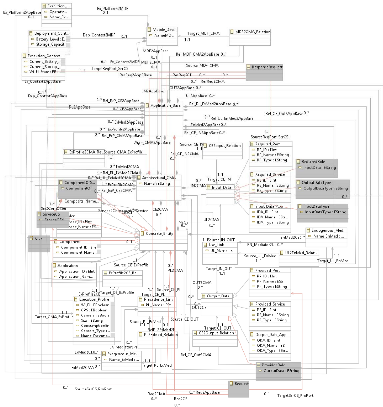
Figure 4 HMA-AD metamodel.ecore
