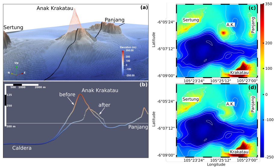
Fig. 7 a Pre and post-collapse topo-bathymetry of Anak Krakatau volcano (dotted grid in transparency illustrating the pre-collapse volcanic edifice); b Cross-section of the pre-collapse (solid line) and post-collapse (dotted line) topo-bathymetry following the black line in a . The water surface at rest is represented by the horizontal white line. There is a \times 5 vertical exaggeration. The scale in a and b is the same and only the view angle changes. Right panels show c pre and d post-collapse topo-bathymetry of Anak Krakatau volcano. Bathymetric contours range from 0 to -250 m every 50 m.
