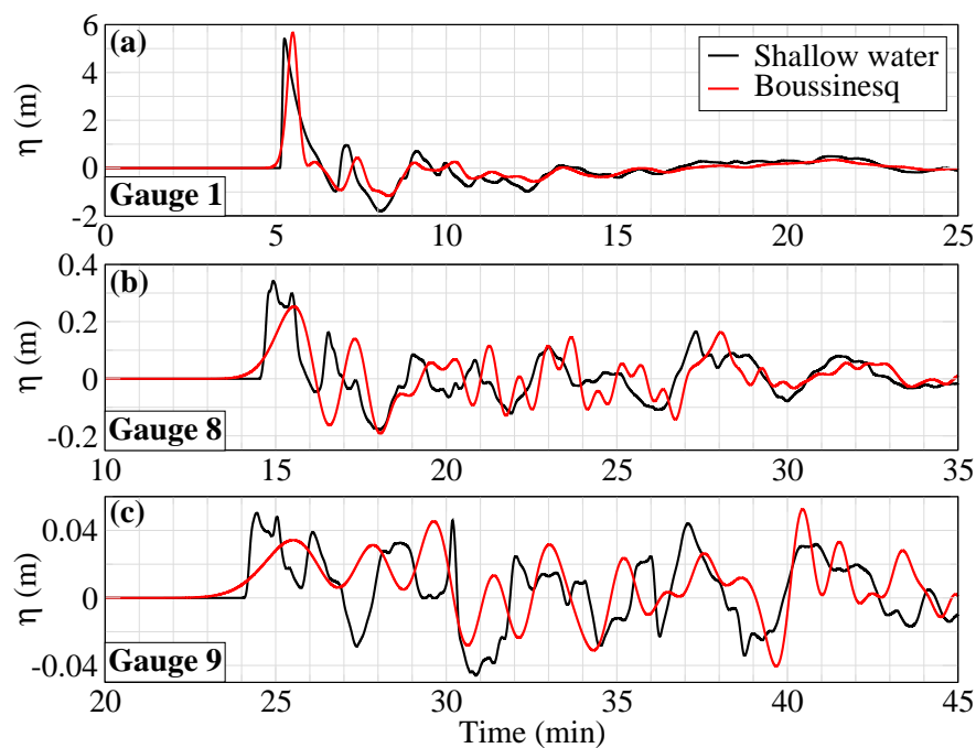
Fig. 12 Comparison of time series calculated by the shallow water (in black) and the Boussinesq (in red) models at Gauges a 1, b 8 and c 9 (Figure 9). The water depths of these gauges are: a 100 m, b 1140 m and c 1960 m.
