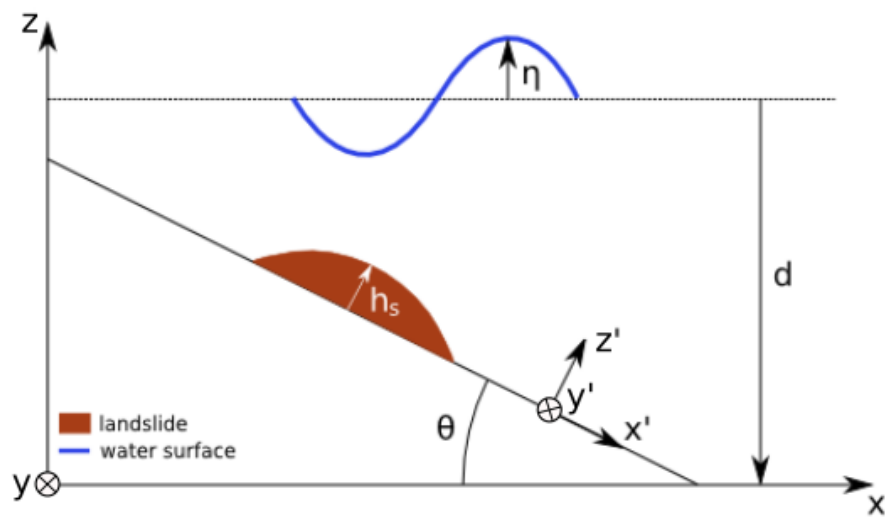
Fig. 5 Definition of parameters used in the AVALANCHE model, with h_s the slide's thickness, \eta the surface elevation, d the depth and \theta the local steepest slope angle.
