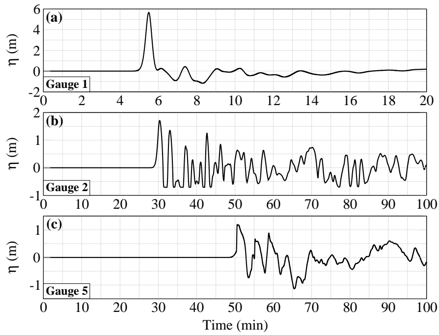
Fig. 11 Computed surface elevations (m) a near the Anak Krakatau volcano, b at Tanjung Lesung and c at Kalianda (Gauges 1, 2 and 5, respectively, see Figure 9).
