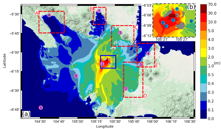
Fig. 9 a Maximum surface elevations computed in Sunda Strait after the collapse of Anak Krakatau volcano. Pink discs with numbers represent the synthetic gauges locations: 10 km away from the volcano (1), at Tanjung Lesung (2), Marina Jambu (3), Ciwandan (4), Kalianda (5), Kota Agung (6), Panjang (7) and the two gauges (8 and 9) used for the comparison between the shallow water and the Boussinesq models. Child grids described in Section 4.3 are represented by the dashed red rectangles. b Close-up of the results around the volcano, corresponding to the blue box in a . Blue discs with numbers represent the synthetic gauges locations used by Grilli et al. (2019).
