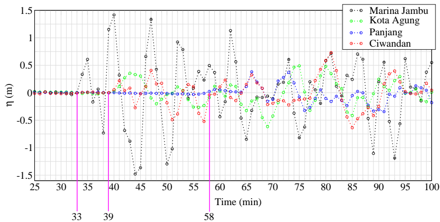
Fig. 4 Time series of surface elevation recorded by tide gauges at Marina Jambu (black), Ciwandan (red), Kota Agung (green) and Panjang (blue) tide gauges (see Figure 9 for locations). Pink lines mark the arrival times at each tide gauges. The arrival times at Kota Agung and Ciwandan are identical.
