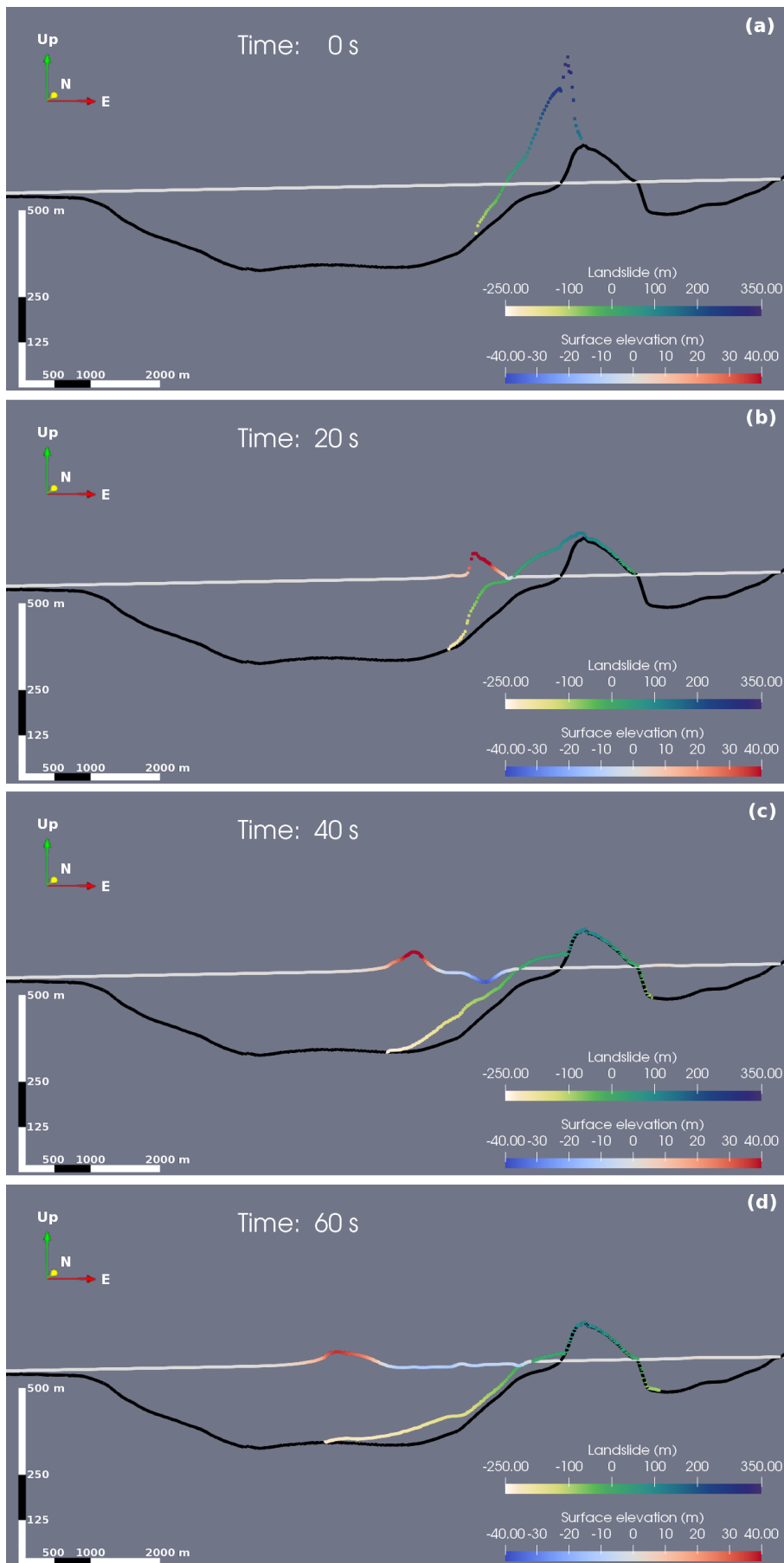
Fig. 8 Snapshots along a W-E cross-section of the simulated water wave (blue to red scale) and landslide (white to dark blue scale) at a t=0 s, b t=20 s, c t=40 s and d t=60 s. The post-collapse topo-bathymetry is represented in black solid line. There is a \times 5 vertical exaggeration.
