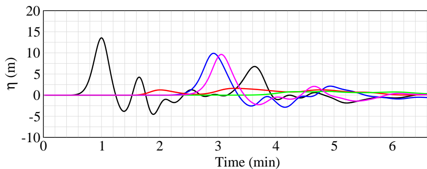
Fig. 13 Time series of surface elevation calculated in the near-field by our model (150 million \text{m}^3 and the code AVALANCHE) at the Gauges 5' (black), 6' (blue), 7' (red), 8' (green) and 9' (magenta) used by Grilli et al. (2019) and presented in Figure 9b. Results are very similar to those presented in Figure 5e of Grilli et al. (2019).
