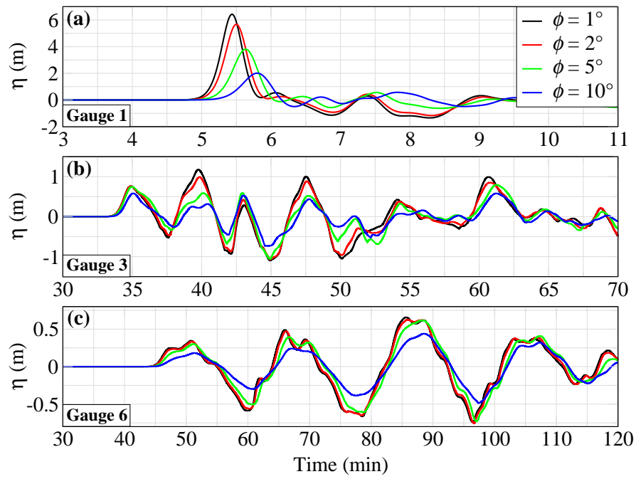
Fig. 6 Time series calculated a at Gauge 1 near the Anak Krakatau volcano, b at Marina Jambu tide gauge (Gauge 3) and c at Kota Agung tide gauge (Gauge 6), using friction angles \phi of 1^\circ (black line), 2^\circ (red line), 5^\circ (green line) and 10^\circ (blue line).
