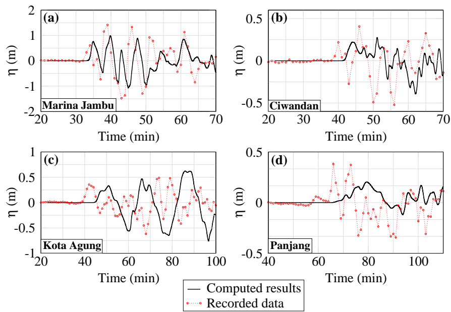
Fig. 10 Comparison between recorded data (in red) and simulated water surface elevations (in black) at a Marina Jambu, b Ciwandan, c Kota Agung and d Panjang (Gauges 3, 4, 6 and 7, respectively, see Figure 9).
