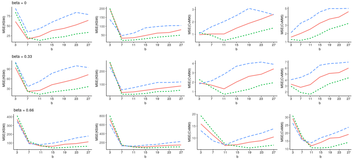
Fig. 4: Empirical MSEs ( \times 10^4 ) of subsampling-based estimators of the 90% and 95%-quantiles of KS(\hat{C}_n) and CvM(\hat{C}_n) against b , for C a bivariate Gumbel–Hougaard copula, \tau = 0.33 , n \in \{50, 100, 200\} and \beta \in \{0, 0.33, 0.66\} .
