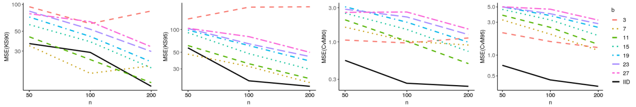
Fig. 5: Empirical MSEs ( \times 10^4 ) of subsampling-based estimators of the 90% and 95%-quantiles of KS(\hat{C}_n) and CvM(\hat{C}_n) against n , for C a bivariate Gumbel–Hougaard copula, \tau = 0.33 , \beta = 0 and b \in \{3, 7, 11, 15, 19, 23, 27\} . The solid lines give the empirical MSEs obtained in the case of subsampling for i.i.d. observations.
