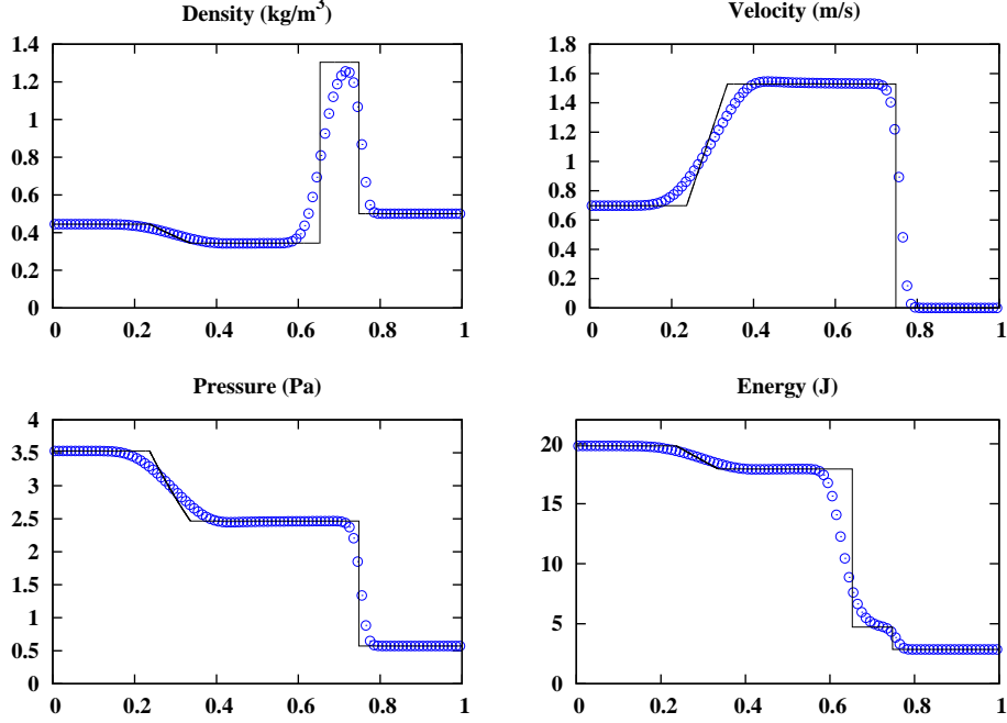
Fig. 42. Test 3 of Sec. 5.2. AUSM + -up scheme with K_p = 0.25 , K_v = 0 and f_c given by Eq. (24) (see Appendix A) ( \circ ), and exact (solid line) solutions at time t = 0.1 s.
