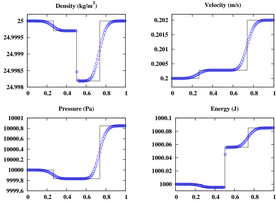
Fig. 4. Low Mach number Riemann problem of Sec. 5.1.1. AUSM + -up scheme with f_c = 1 ( \circ ) and exact (solid line) solutions at time t = 0.01 s.
