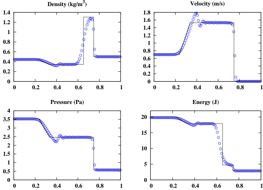
Fig. 38. Test 3 of Sec. 5.2. AUSM-IT scheme with K_p = 0 and K_I = 0.25 ( \circ ) and exact (solid line) solutions at time t = 0.1 s.
