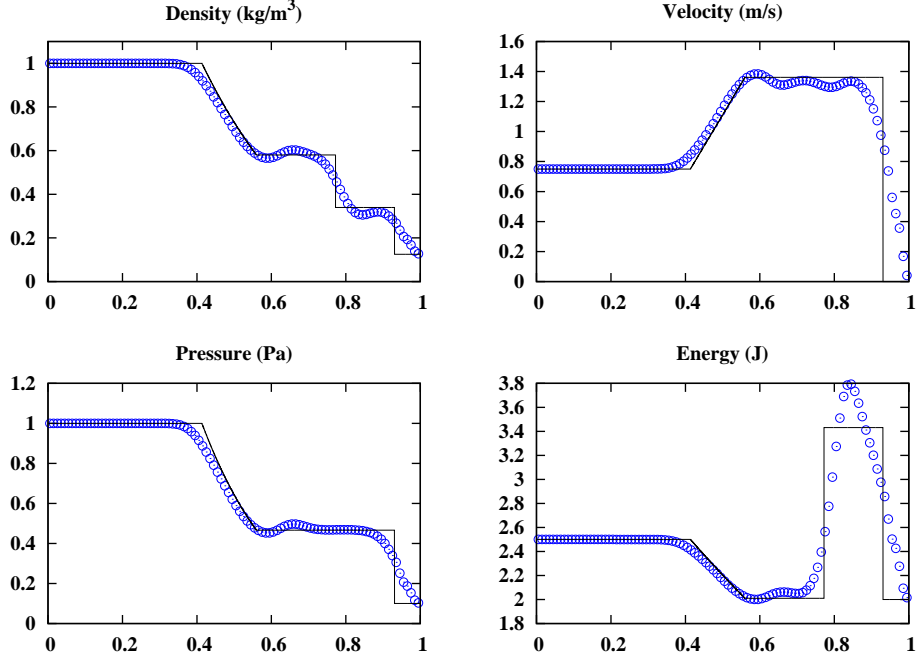
Fig. 30. Test 1 of Sec. 5.2. Momentum interpolation scheme ( \circ ) (see Eq. (29)) and exact (solid line) solutions at time t = 0.2 s.
