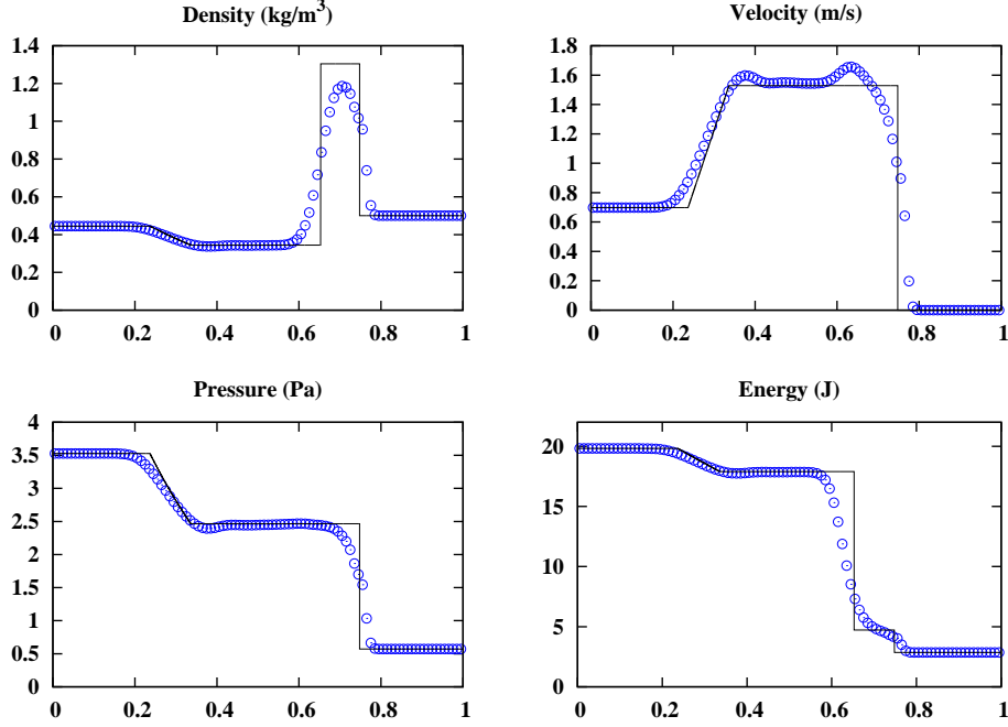
Fig. 46. Test 3 of Sec. 5.2. Momentum interpolation scheme ( \circ ) (see Eq. (29)) and exact (solid line) solutions at time t = 0.1 s.
