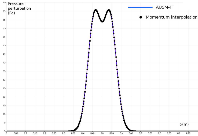
Fig. 19. Two-dimensional acoustic pulse propagation, cf. Sec. 5.1.4. Distribution of the pressure perturbation profiles at t = 0.1 ms for y = 0.5 m (white line in Fig. 18) by the AUSM-IT scheme (solid line) and the momentum interpolation method ( \bullet ).
