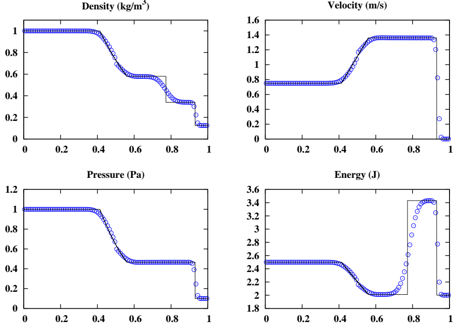
Fig. 26. Test 1 of Sec. 5.2. AUSM + -up scheme with K_p = 0.25 , K_v = 0 and f_c given by Eq. (24) (see Appendix A) ( \circ ), and exact (solid line) solutions at time t = 0.2 s.
