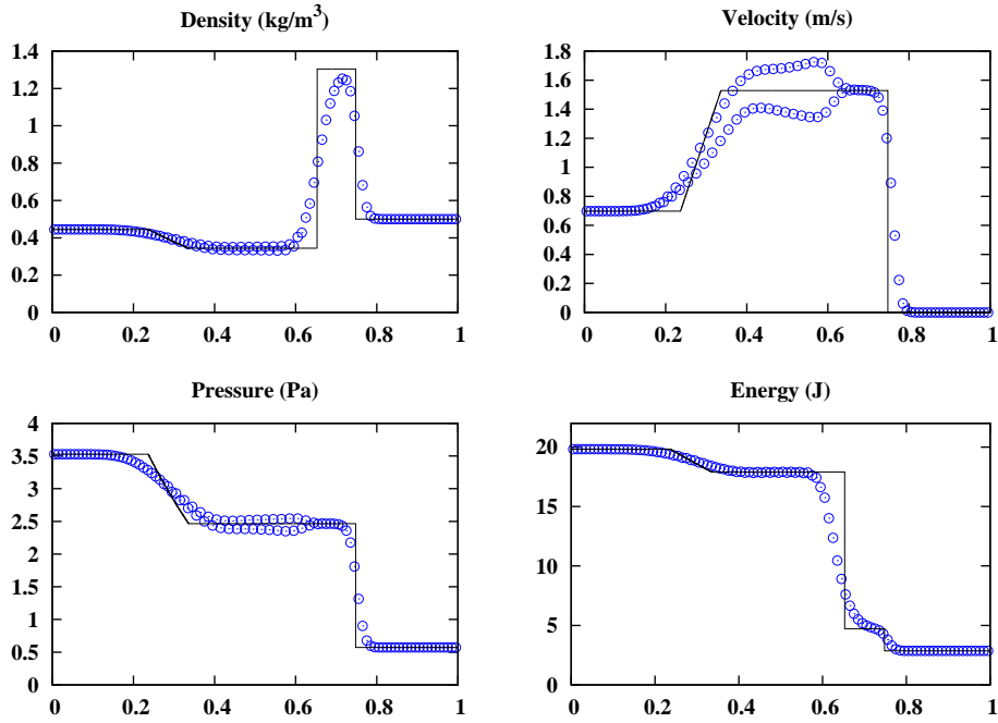
Fig. 40. Test 3 of Sec. 5.2. AUSM + -up scheme with K_p = 0.25 , K_v = 0.75 and f_c given by Eq. (24) (see Appendix A) ( \circ ), and exact (solid line) solutions at time t = 0.1 s.
