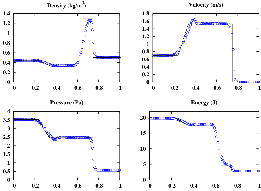
Fig. 39. Test 3 of Sec. 5.2. AUSM + scheme ( \circ ) and exact (solid line) solutions at time t = 0.1 s.
