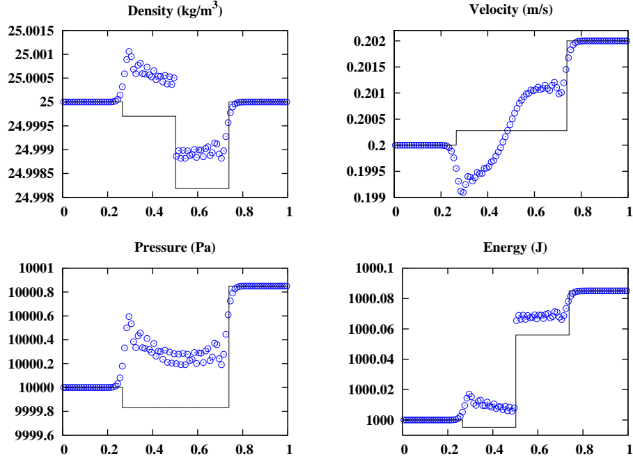
Fig. 5. Low Mach number Riemann problem of Sec. 5.1.1. Momentum interpolation ( \circ ) and exact (solid line) solutions at time t = 0.01 s.
