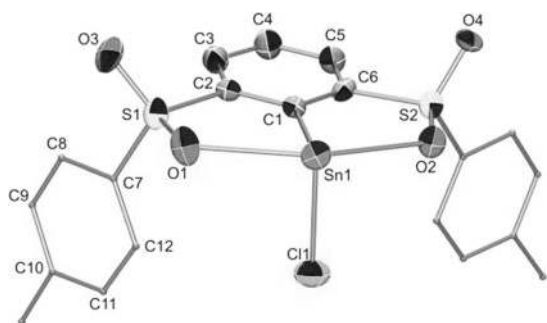
Figure 3. Molecular structure of compound 3 -CH 2 Cl 2 in the solid state (ball-and-stick model). Thermal ellipsoids were set at 50% probability. For clarity, hydrogen atoms and the co-crystallized solvent molecules are omitted and tolyl groups are simplified by representation as a stick model. Selected bond distances [Å] and bond angles [°]: S1–O1 1.455(7), S1–O3 1.434(7), S2–O2 1.452(7), S2–O4 1.460(7), Sn1–O1 2.458(7), Sn1–O2 2.543(7), Sn1–Cl1 2.454(3); O1–S1–O3 118.7(4), O2–S2–O4 117.3(4), O1–S1–C2 105.1(4), C1–Sn1–Cl1 91.1(2), C1–Sn1–O1 73.2(3), O1–Sn1–O2 145.1(2).
