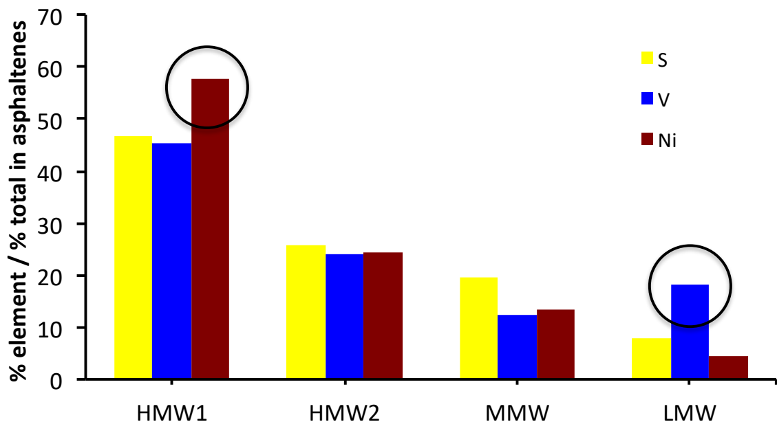
Figure 7. Percentage distributions of the V, Ni and S compounds in the separated fractions of the asphaltene.
