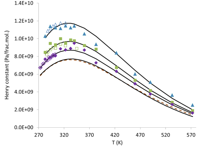
Fig. 5. Henry constant of H 2 in aqueous NaCl solutions versus temperature. Open symbols: experimental data in salted water. Filled symbols: Monte Carlo simulation results (diamonds: NaCl = 0.5 mol/kg H2O , squares: NaCl = 1 mol/kg H2O , triangles: NaCl = 2 mol/kg H2O ). Dashed red line: pure water correlation (Eq. (3)). Solid black lines: Calibrated SW equation of state.
