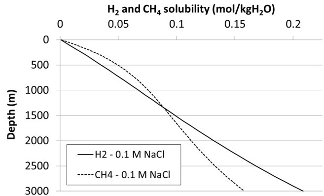
Fig. 8. Hydrogen and methane solubility versus depth for NaCl concentrations of 0.1 mol/kg H 2 O .
